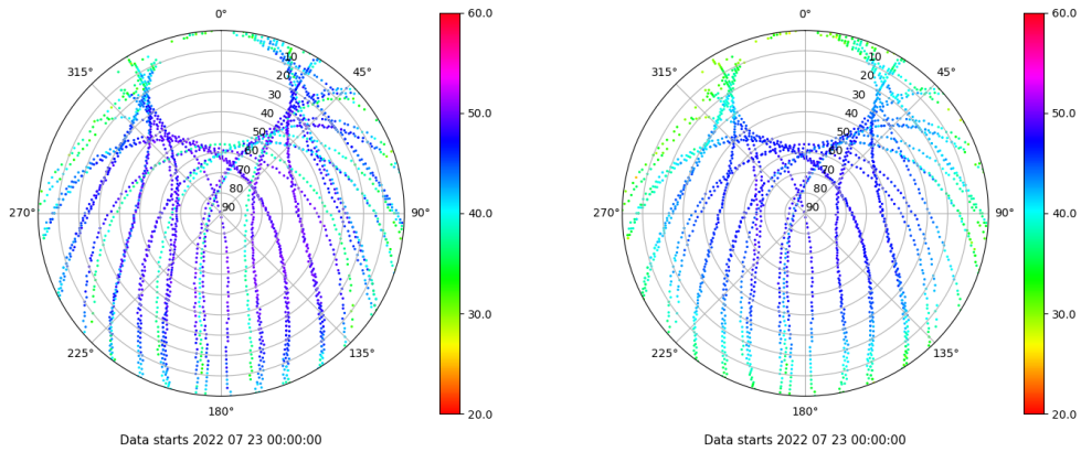
Skyplot for station YEB1. Signal to Noise S1C Data file YEB100ESP_R_2022204.xtr Skyplot for station YEB1. Signal to Noise S2P Data file YEB100ESP_R_2022204.xtr
