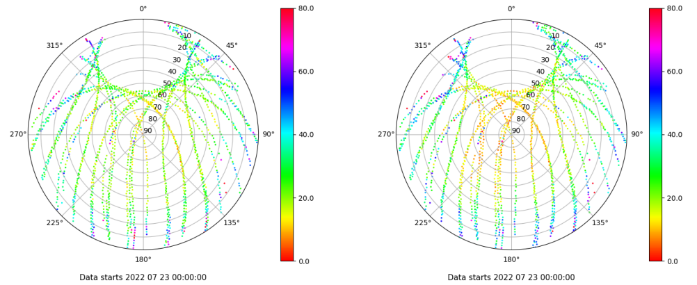
Skyplot for station YEB1. Parameter M1C Data file YEB100ESP_R_2022204.xtr Skyplot for station YEB1. Parameter M2P Data file YEB100ESP_R_2022204.xtr
