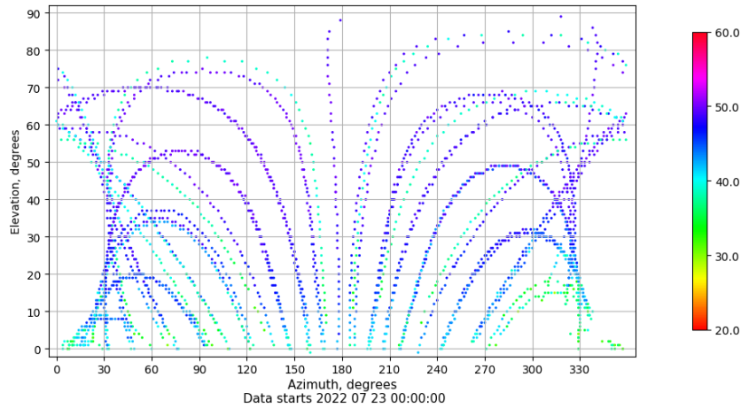
Azimuth-elevation plot for station YEB1. Signal to Noise S1C Data file YEB100ESP_R_2022204.xtr
