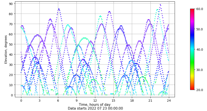
Time-elevation plot for station YEB1. Signal to Noise S1C Data file YEB100ESP_R_2022204.xtr
