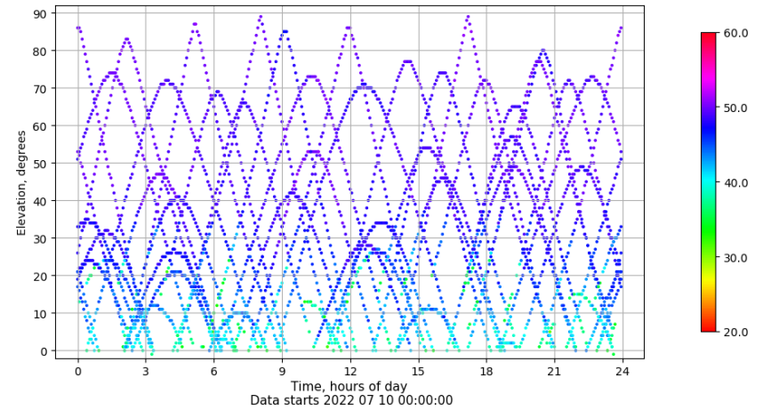
Time-elevation plot for station YEB1. Signal to Noise S1C Data file YEB100ESP_R_2022191.xtr
