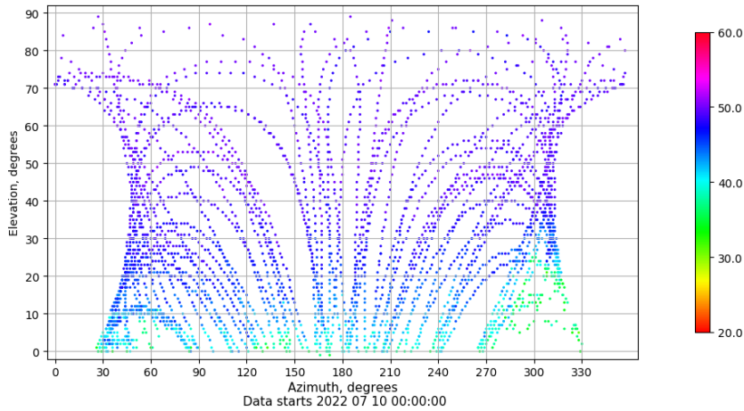
Azimuth-elevation plot for station YEB1. Signal to Noise S1C Data file YEB100ESP_R_2022191.xtr
