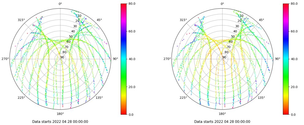
Skyplot for station YEB1. Parameter M1C Data file YEB100ESP_R_2022118.xtr Skyplot for station YEB1. Parameter M2P Data file YEB100ESP_R_2022118.xtr
