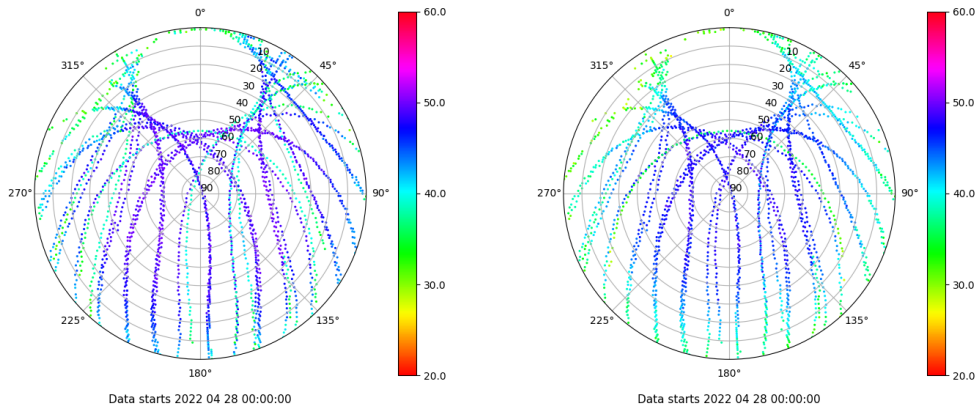
Skyplot for station YEB1. Signal to Noise S1C Data file YEB100ESP_R_2022118.xtr Skyplot for station YEB1. Signal to Noise S2P Data file YEB100ESP_R_2022118.xtr
