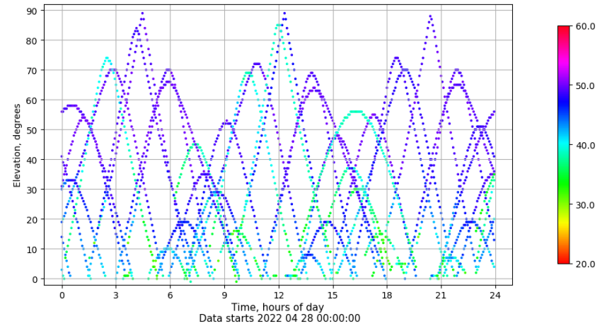
Time-elevation plot for station YEB1. Signal to Noise S1C Data file YEB100ESP_R_2022118.xtr
