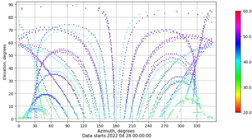
Azimuth-elevation plot for station YEB1. Signal to Noise S1C Data file YEB100ESP_R_2022118.xtr
