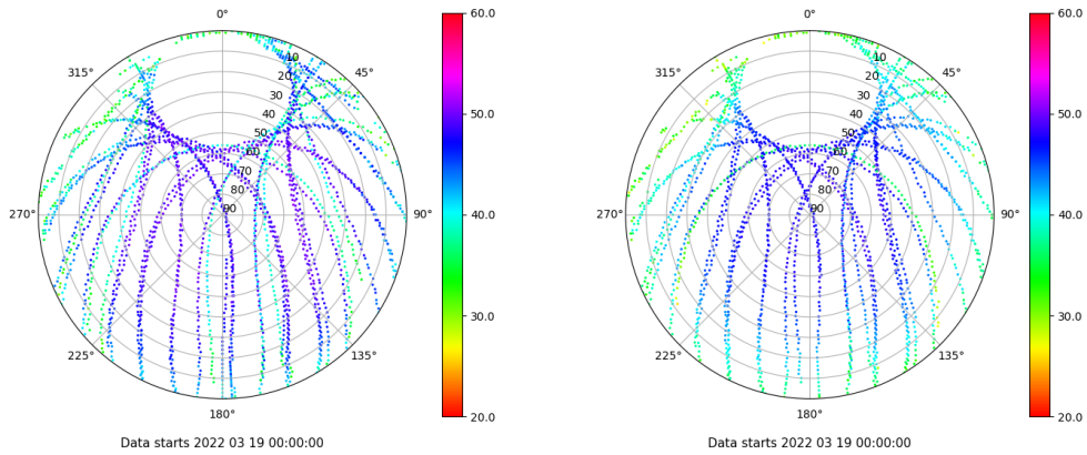
Skyplot for station YEB1. Signal to Noise S1C Data file YEB100ESP_R_2022078.xtr Skyplot for station YEB1. Signal to Noise S2P Data file YEB100ESP_R_2022078.xtr
