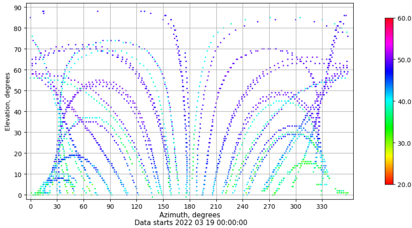
Azimuth-elevation plot for station YEB1. Signal to Noise S1C Data file YEB100ESP_R_2022078.xtr
