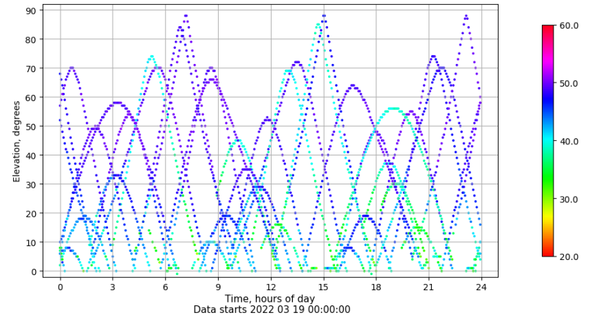
Time-elevation plot for station YEB1. Signal to Noise S1C Data file YEB100ESP_R_2022078.xtr
