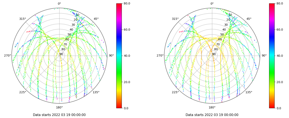
Skyplot for station YEB1. Parameter M1C Data file YEB100ESP_R_2022078.xtr Skyplot for station YEB1. Parameter M2P Data file YEB100ESP_R_2022078.xtr
