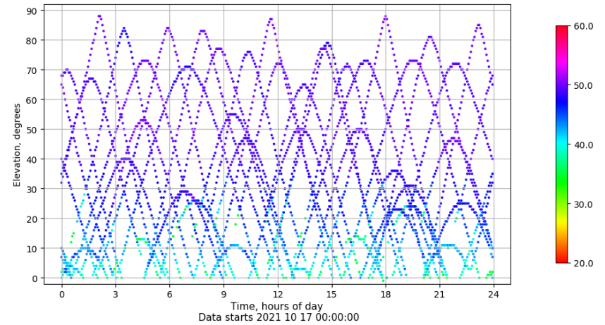
Time-elevation plot for station YEB1. Signal to Noise S1C Data file YEB100ESP_R_2021290.xtr
