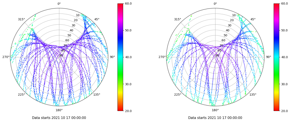
Skyplot for station YEB1. Signal to Noise S1C Data file YEB100ESP_R_2021290.xtr Skyplot for station YEB1. Signal to Noise S2S Data file YEB100ESP_R_2021290.xtr
