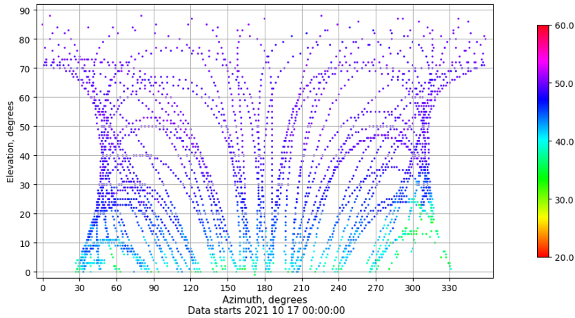
Azimuth-elevation plot for station YEB1. Signal to Noise S1C Data file YEB100ESP_R_2021290.xtr
