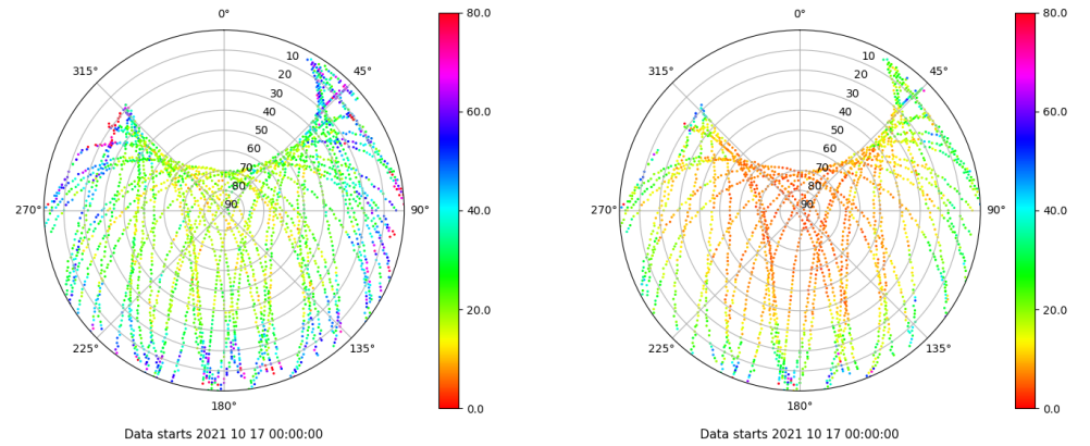
Skyplot for station YEB1. Parameter M1C Data file YEB100ESP_R_2021290.xtr Skyplot for station YEB1. Parameter M2S Data file YEB100ESP_R_2021290.xtr
