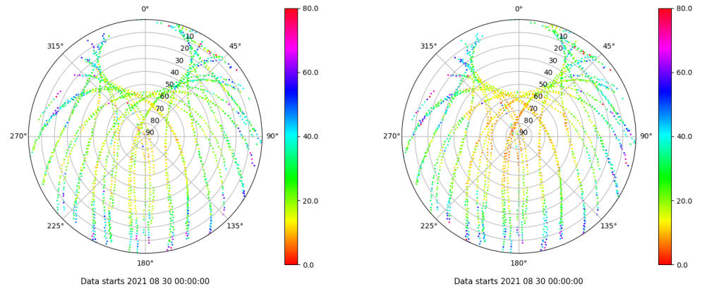
Skyplot for station YEB1. Parameter M1C Data file YEB100ESP_R_2021242.xtr Skyplot for station YEB1. Parameter M2P Data file YEB100ESP_R_2021242.xtr
