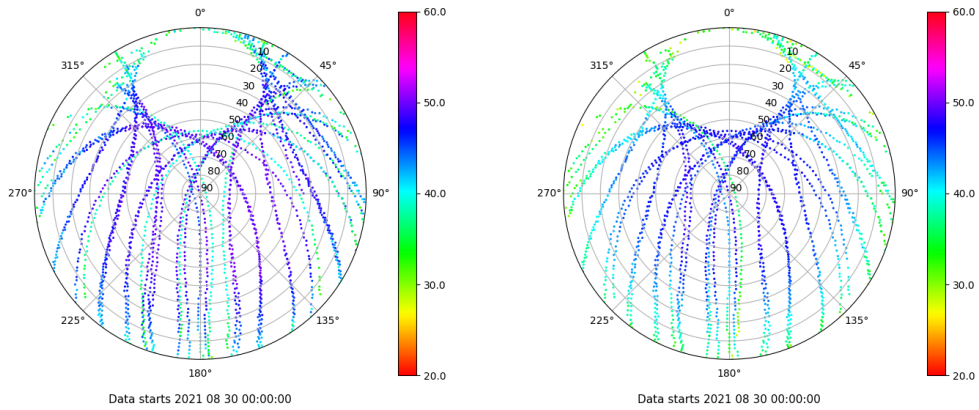
Skyplot for station YEB1. Signal to Noise S1C Data file YEB100ESP_R_2021242.xtr Skyplot for station YEB1. Signal to Noise S2P Data file YEB100ESP_R_2021242.xtr
