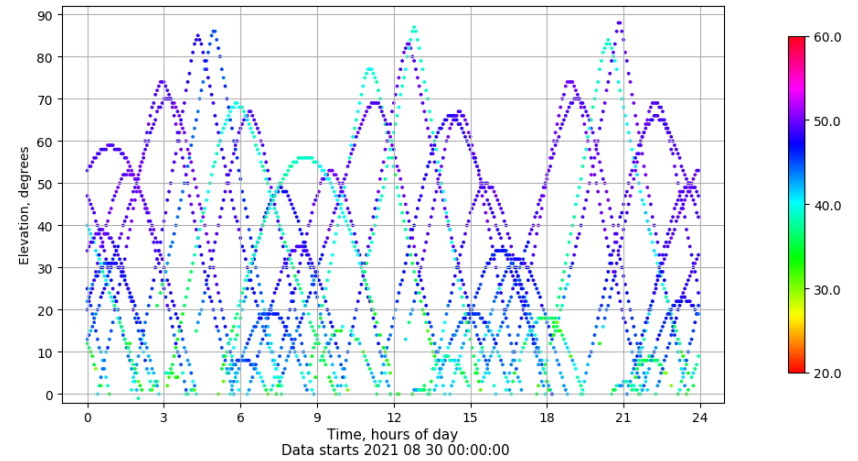
Time-elevation plot for station YEB1. Signal to Noise S1C Data file YEB100ESP_R_2021242.xtr
