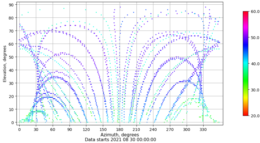
Azimuth-elevation plot for station YEB1. Signal to Noise S1C Data file YEB100ESP_R_2021242.xtr
