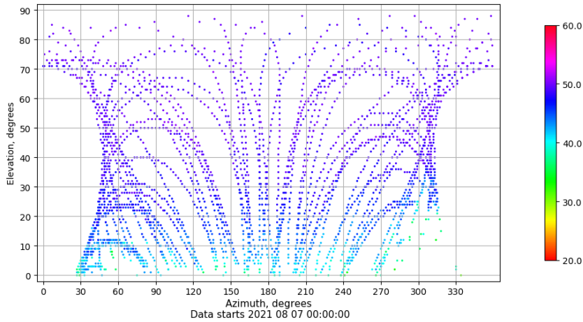
Azimuth-elevation plot for station YEB1. Signal to Noise S1C Data file YEB100ESP_R_2021219.xtr
