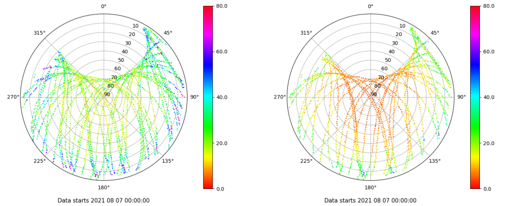
Skyplot for station YEB1. Parameter M1C Data file YEB100ESP_R_2021219.xtr Skyplot for station YEB1. Parameter M2S Data file YEB100ESP_R_2021219.xtr
