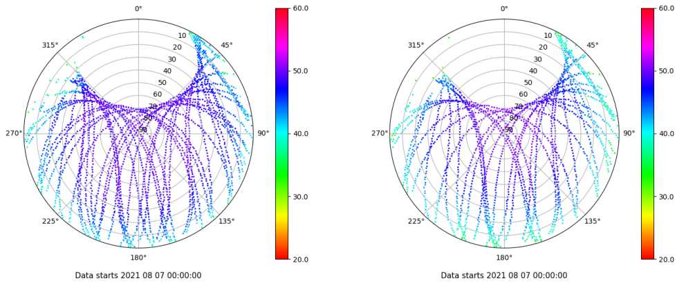
Skyplot for station YEB1. Signal to Noise S1C Data file YEB100ESP_R_2021219.xtr Skyplot for station YEB1. Signal to Noise S2S Data file YEB100ESP_R_2021219.xtr
