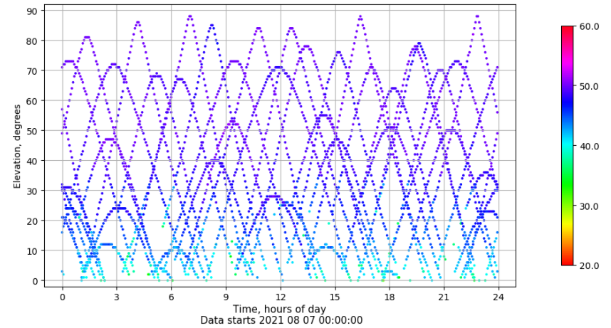
Time-elevation plot for station YEB1. Signal to Noise S1C Data file YEB100ESP_R_2021219.xtr
