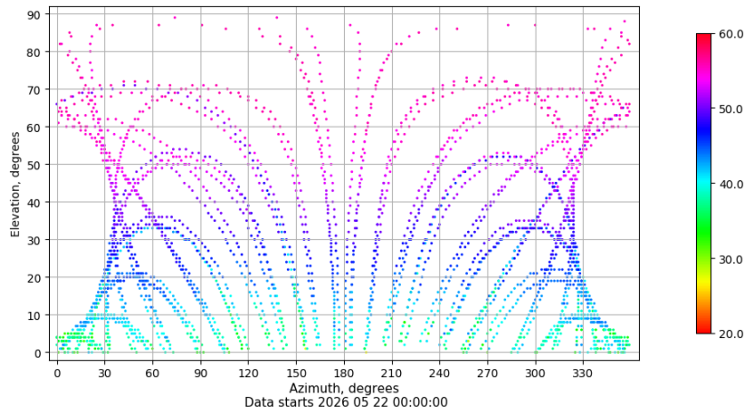
Azimuth-elevation plot for station XIXO. Signal to Noise S1C Data file XIXO00ESP_R_2026142.xtr
