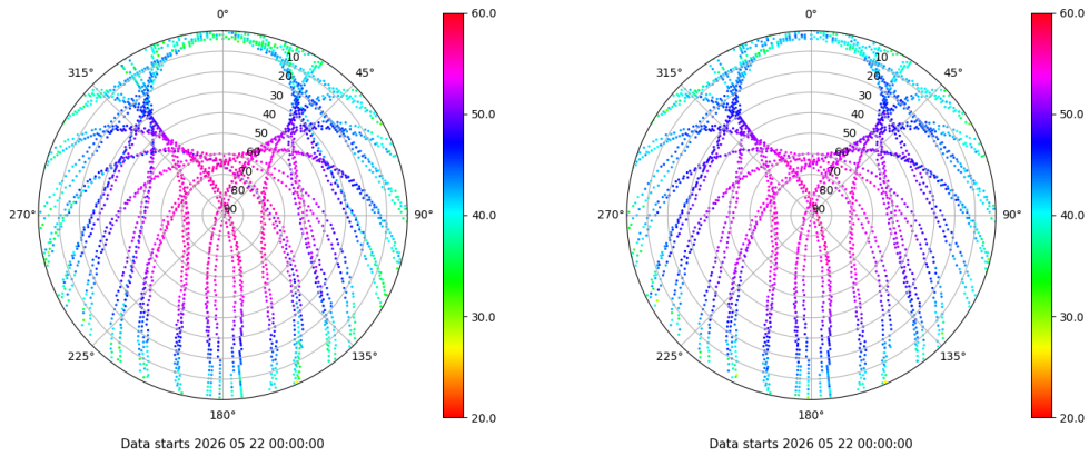
Skyplot for station XIXO. Signal to Noise S1C Data file XIXO00ESP_R_2026142.xtr Skyplot for station XIXO. Signal to Noise S2C Data file XIXO00ESP_R_2026142.xtr
