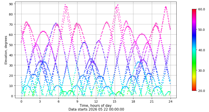
Time-elevation plot for station XIXO. Signal to Noise S1C Data file XIXO00ESP_R_2026142.xtr
