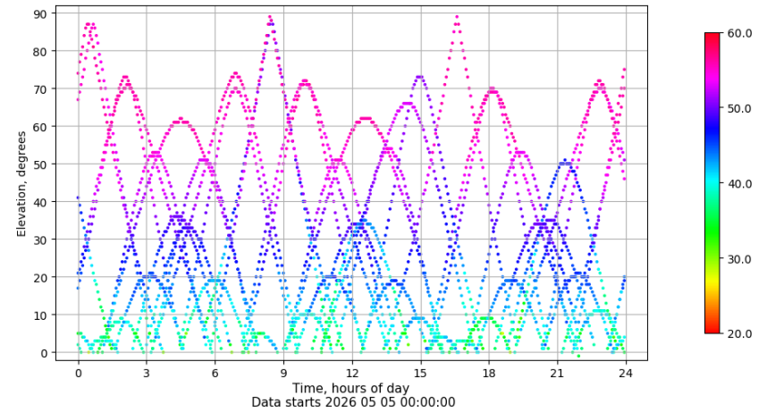
Time-elevation plot for station XIXO. Signal to Noise S1C Data file XIXO00ESP_R_2026125.xtr
