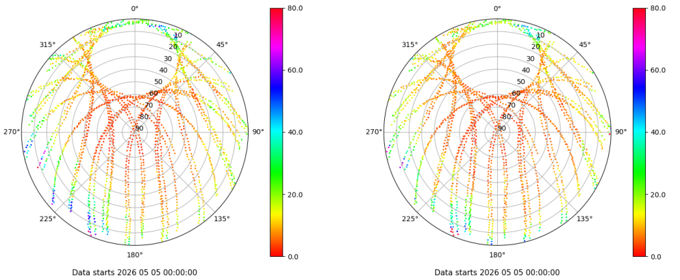
Skyplot for station XIXO. Parameter M1C Data file XIXO00ESP_R_2026125.xtr Skyplot for station XIXO. Parameter M2C Data file XIXO00ESP_R_2026125.xtr
