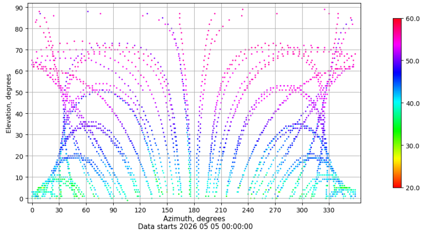
Azimuth-elevation plot for station XIXO. Signal to Noise S1C Data file XIXO00ESP_R_2026125.xtr
