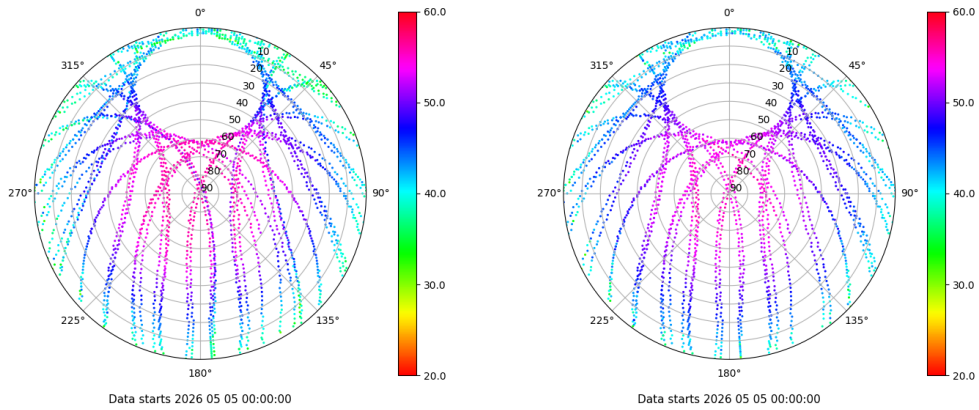
Skyplot for station XIXO. Signal to Noise S1C Data file XIXO00ESP_R_2026125.xtr Skyplot for station XIXO. Signal to Noise S2C Data file XIXO00ESP_R_2026125.xtr
