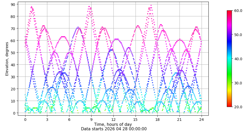
Time-elevation plot for station XIXO. Signal to Noise S1C Data file XIXO00ESP_R_2026118.xtr
