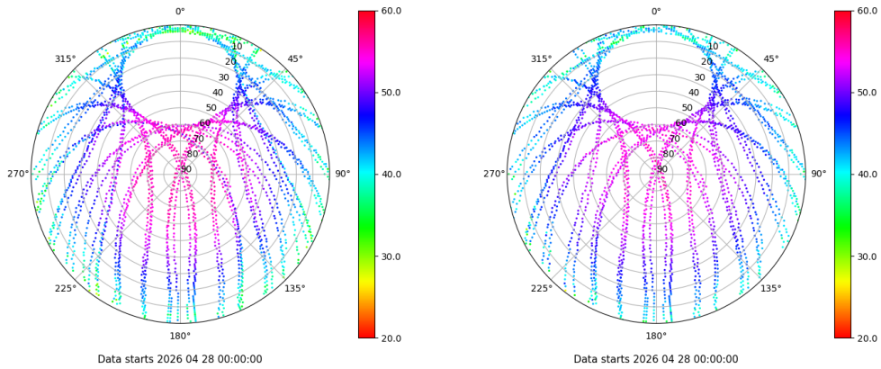
Skyplot for station XIXO. Signal to Noise S1C Data file XIXO00ESP_R_2026118.xtr Skyplot for station XIXO. Signal to Noise S2C Data file XIXO00ESP_R_2026118.xtr
