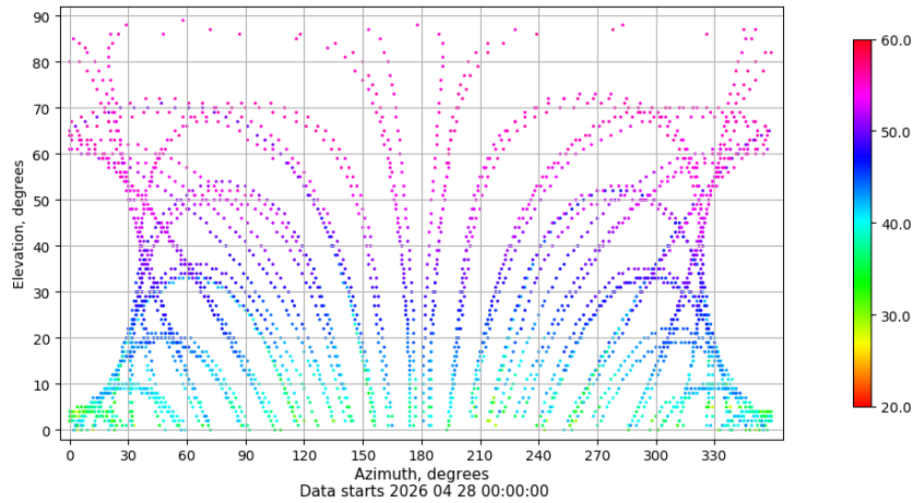
Azimuth-elevation plot for station XIXO. Signal to Noise S1C Data file XIXO00ESP_R_2026118.xtr
