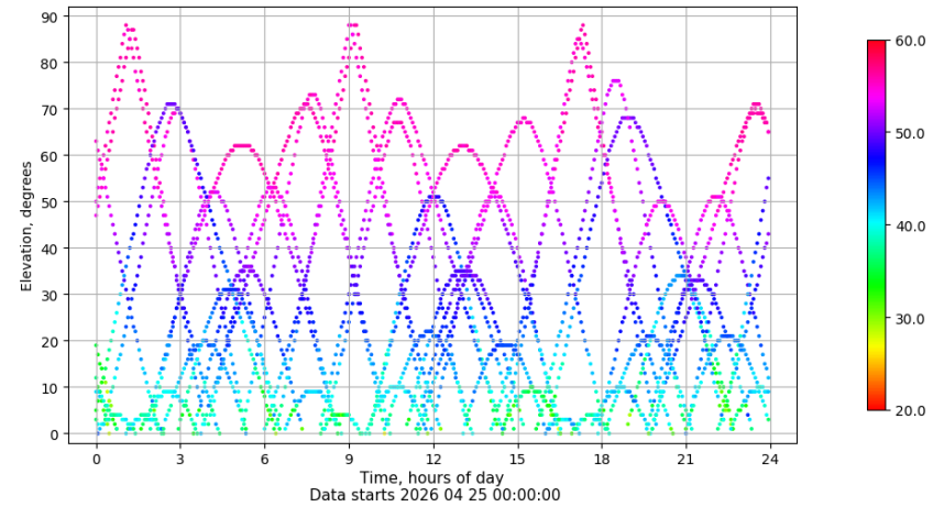
Time-elevation plot for station XIXO. Signal to Noise S1C Data file XIXO00ESP_R_2026115.xtr
