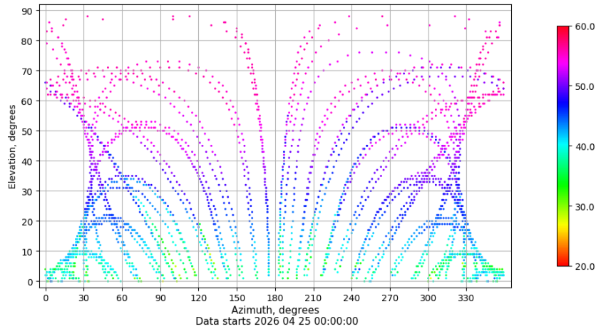
Azimuth-elevation plot for station XIXO. Signal to Noise S1C Data file XIXO00ESP_R_2026115.xtr
