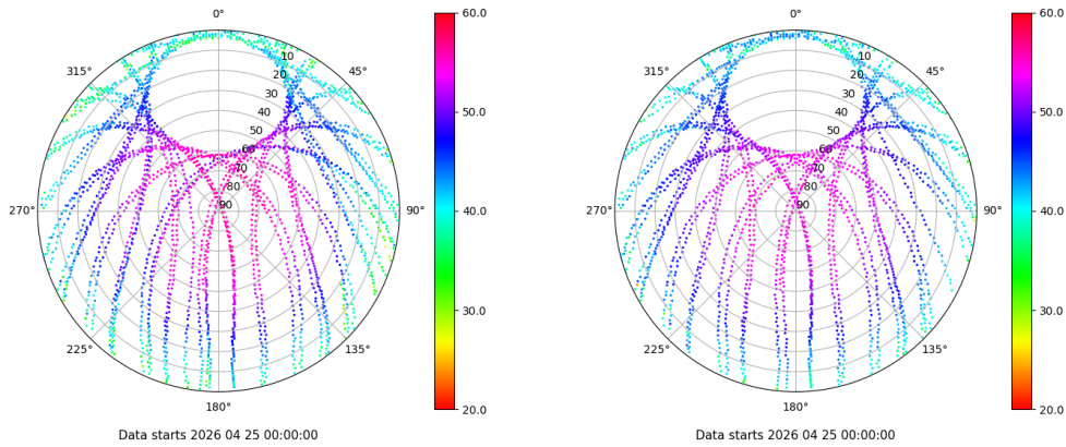
Skyplot for station XIXO. Signal to Noise S1C Data file XIXO00ESP_R_2026115.xtr Skyplot for station XIXO. Signal to Noise S2C Data file XIXO00ESP_R_2026115.xtr
