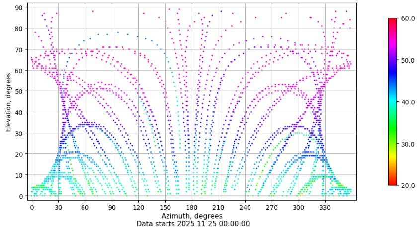
Azimuth-elevation plot for station XIXO. Signal to Noise S1C Data file XIXO00ESP_R_2025329.xtr
