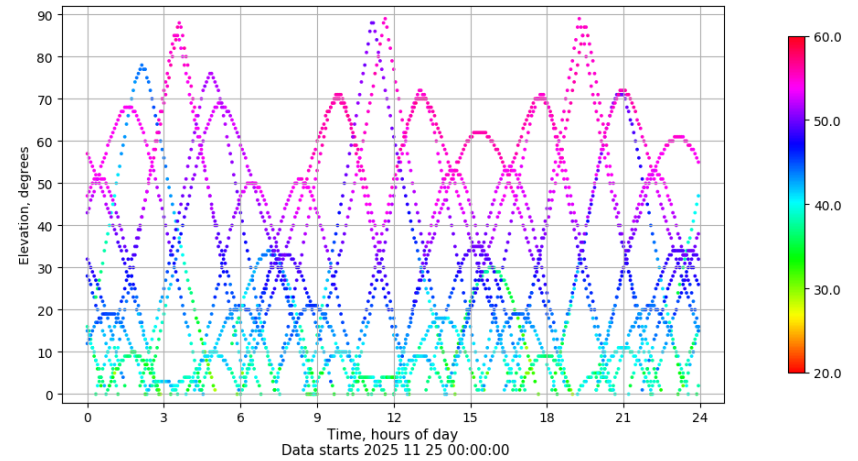
Time-elevation plot for station XIXO. Signal to Noise S1C Data file XIXO00ESP_R_2025329.xtr
