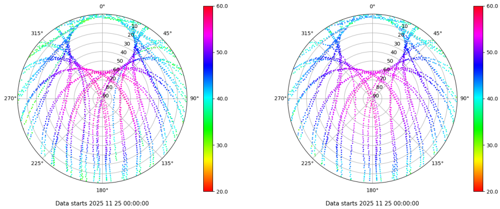
Skyplot for station XIXO. Signal to Noise S1C Data file XIXO00ESP_R_2025329.xtr Skyplot for station XIXO. Signal to Noise S2C Data file XIXO00ESP_R_2025329.xtr
