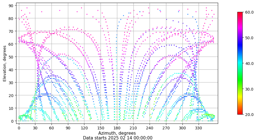
Azimuth-elevation plot for station XIXO. Signal to Noise S1C Data file XIXO00ESP_R_2025045.xtr
