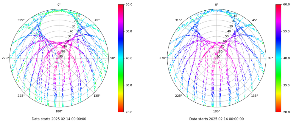
Skyplot for station XIXO. Signal to Noise S1C Data file XIXO00ESP_R_2025045.xtr Skyplot for station XIXO. Signal to Noise S2C Data file XIXO00ESP_R_2025045.xtr
