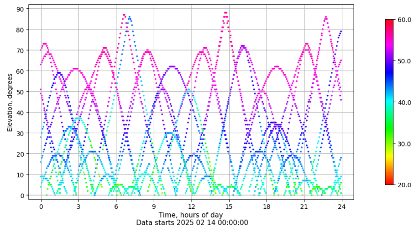
Time-elevation plot for station XIXO. Signal to Noise S1C Data file XIXO00ESP_R_2025045.xtr
