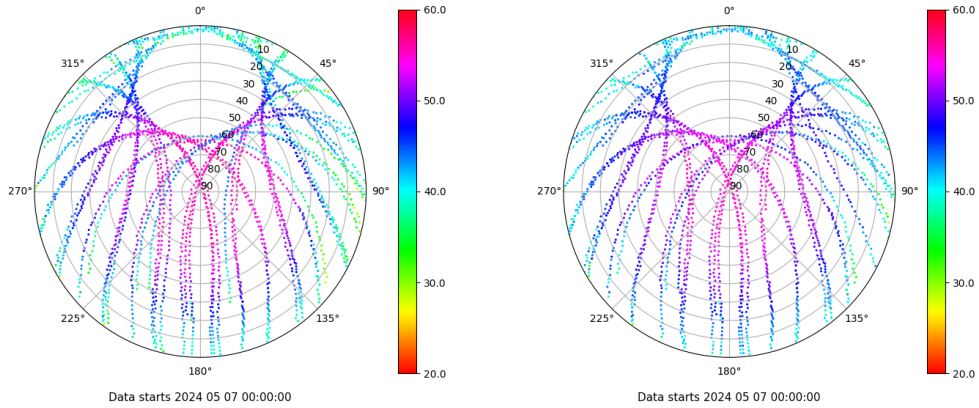
Skyplot for station XIXO. Signal to Noise S1C Data file XIXO00ESP_R_2024128.xtr Skyplot for station XIXO. Signal to Noise S2C Data file XIXO00ESP_R_2024128.xtr
