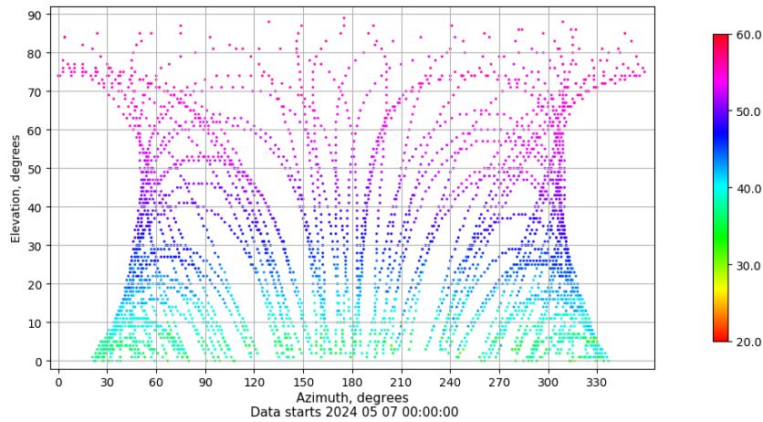
Azimuth-elevation plot for station XIXO. Signal to Noise S1C Data file XIXO00ESP_R_2024128.xtr
