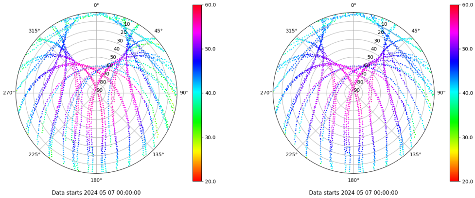
Skyplot for station XIXO. Signal to Noise S1C Data file XIXO00ESP_R_2024128.xtr Skyplot for station XIXO. Signal to Noise S2C Data file XIXO00ESP_R_2024128.xtr
