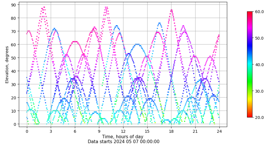
Time-elevation plot for station XIXO. Signal to Noise S1C Data file XIXO00ESP_R_2024128.xtr
