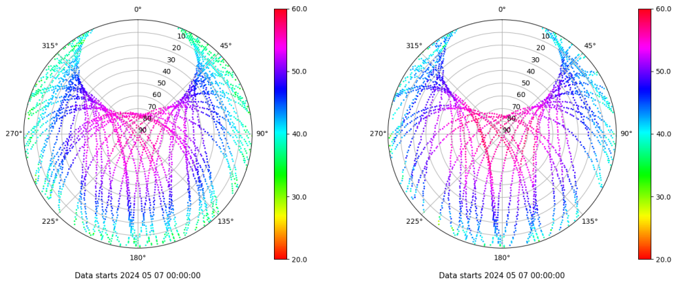
Skyplot for station XIXO. Signal to Noise S1C Data file XIXO00ESP_R_2024128.xtr Skyplot for station XIXO. Signal to Noise S2S Data file XIXO00ESP_R_2024128.xtr
