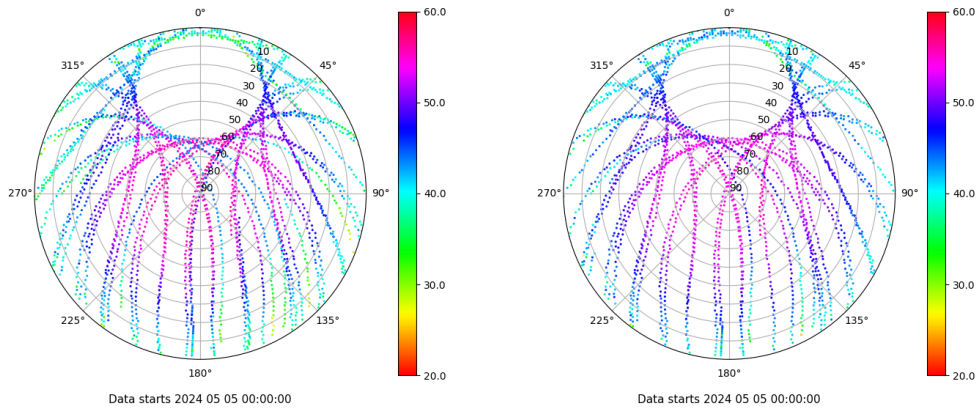
Skyplot for station XIXO. Signal to Noise S1C Data file XIXO00ESP_R_2024126.xtr Skyplot for station XIXO. Signal to Noise S2C Data file XIXO00ESP_R_2024126.xtr
