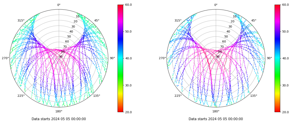
Skyplot for station XIXO. Signal to Noise S1C Data file XIXO00ESP_R_2024126.xtr Skyplot for station XIXO. Signal to Noise S2S Data file XIXO00ESP_R_2024126.xtr
