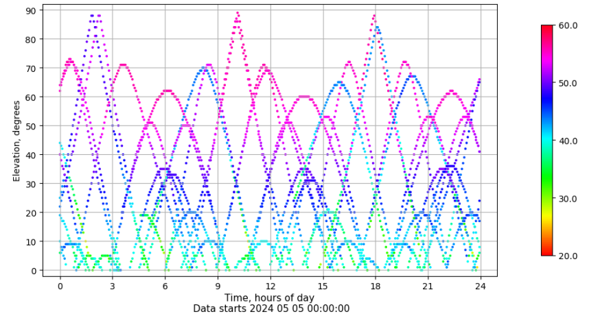
Time-elevation plot for station XIXO. Signal to Noise S1C Data file XIXO00ESP_R_2024126.xtr
