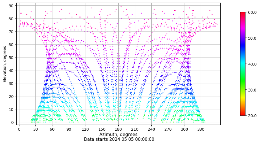
Azimuth-elevation plot for station XIXO. Signal to Noise S1C Data file XIXO00ESP_R_2024126.xtr
