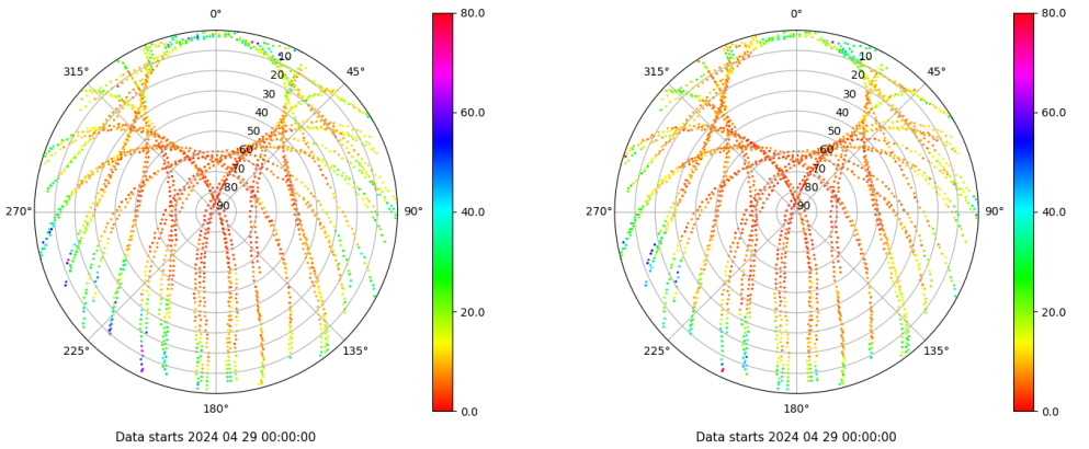
Skyplot for station XIXO. Parameter M1C Data file XIXO00ESP_R_2024120.xtr Skyplot for station XIXO. Parameter M2C Data file XIXO00ESP_R_2024120.xtr
