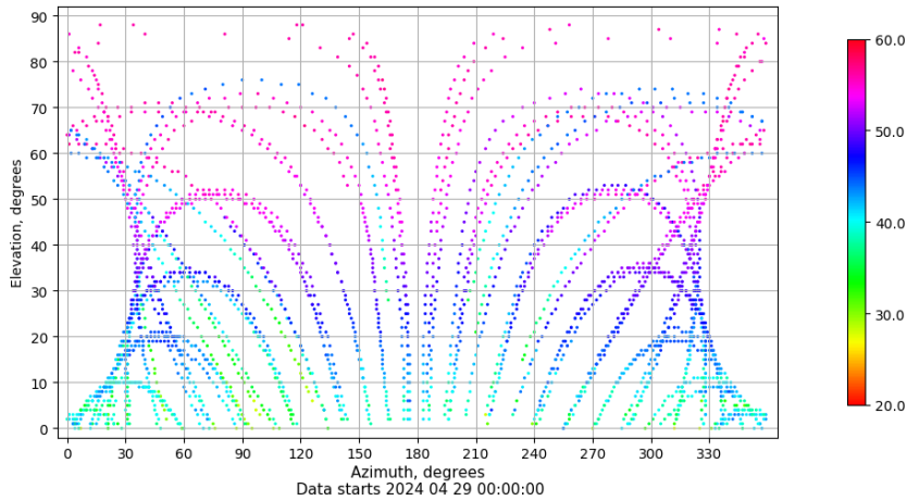
Azimuth-elevation plot for station XIXO. Signal to Noise S1C Data file XIXO00ESP_R_2024120.xtr
