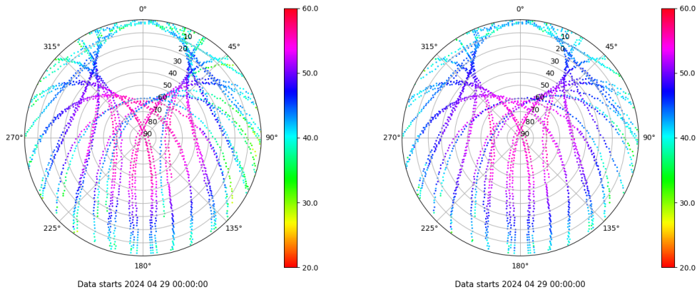
Skyplot for station XIXO. Signal to Noise S1C Data file XIXO00ESP_R_2024120.xtr Skyplot for station XIXO. Signal to Noise S2C Data file XIXO00ESP_R_2024120.xtr
