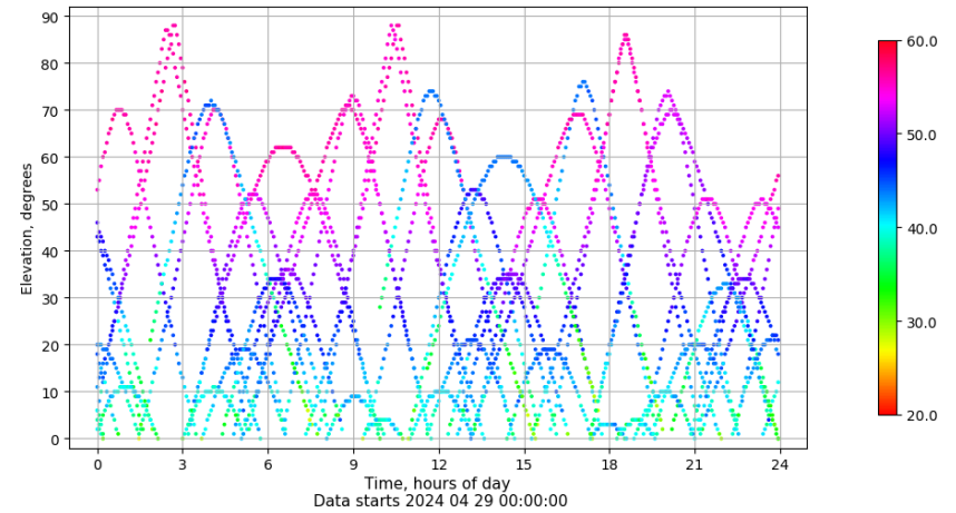
Time-elevation plot for station XIXO. Signal to Noise S1C Data file XIXO00ESP_R_2024120.xtr
