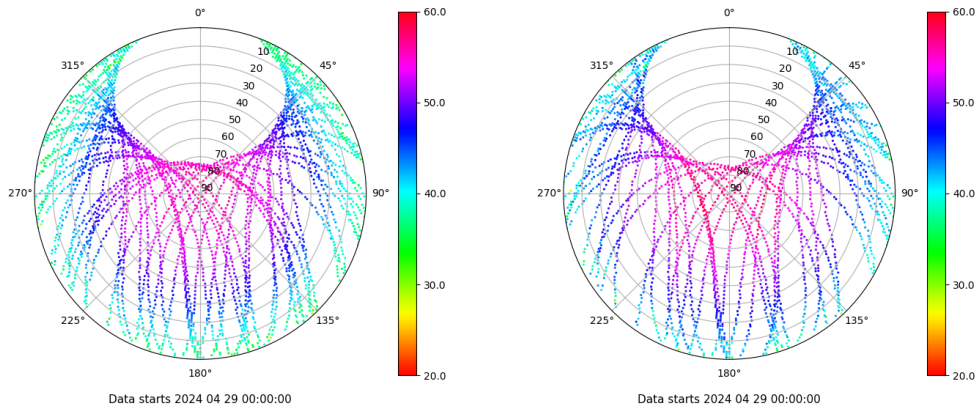
Skyplot for station XIXO. Signal to Noise S1C Data file XIXO00ESP_R_2024120.xtr Skyplot for station XIXO. Signal to Noise S2S Data file XIXO00ESP_R_2024120.xtr
