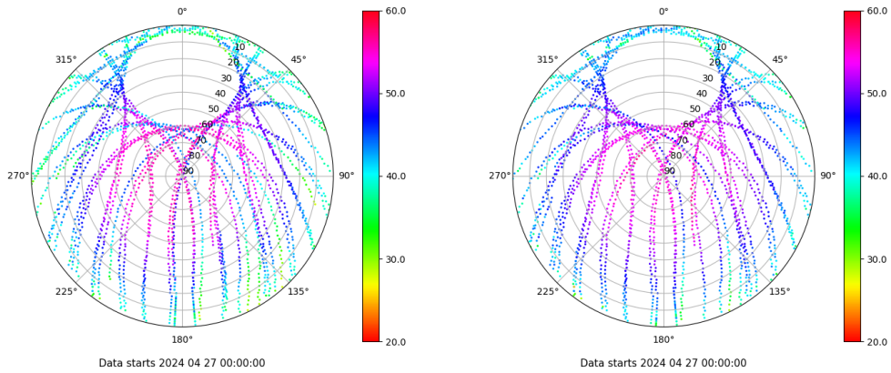
Skyplot for station XIXO. Signal to Noise S1C Data file XIXO00ESP_R_2024118.xtr Skyplot for station XIXO. Signal to Noise S2C Data file XIXO00ESP_R_2024118.xtr
