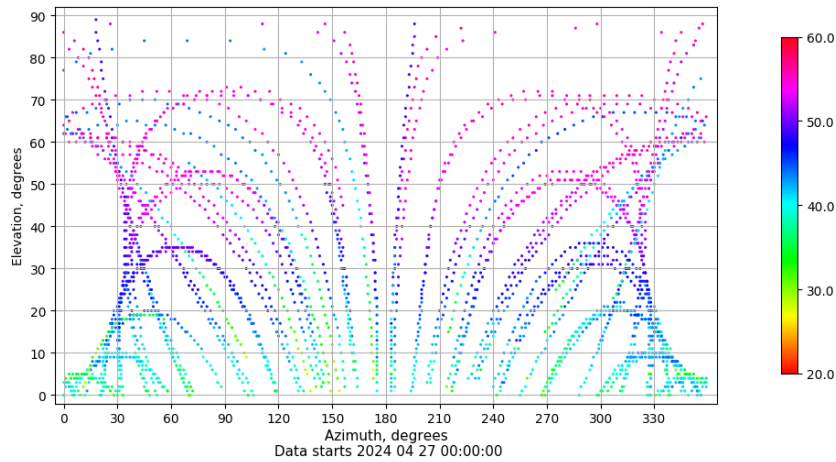
Azimuth-elevation plot for station XIXO. Signal to Noise S1C Data file XIXO00ESP_R_2024118.xtr
