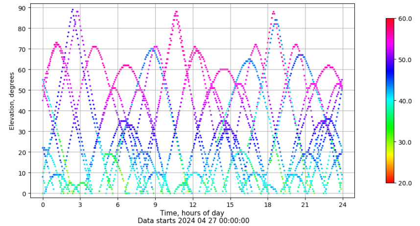
Time-elevation plot for station XIXO. Signal to Noise S1C Data file XIXO00ESP_R_2024118.xtr
