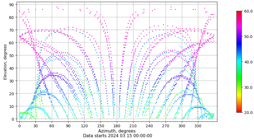
Azimuth-elevation plot for station XIXO. Signal to Noise S1C Data file XIXO00ESP_R_2024075.xtr
