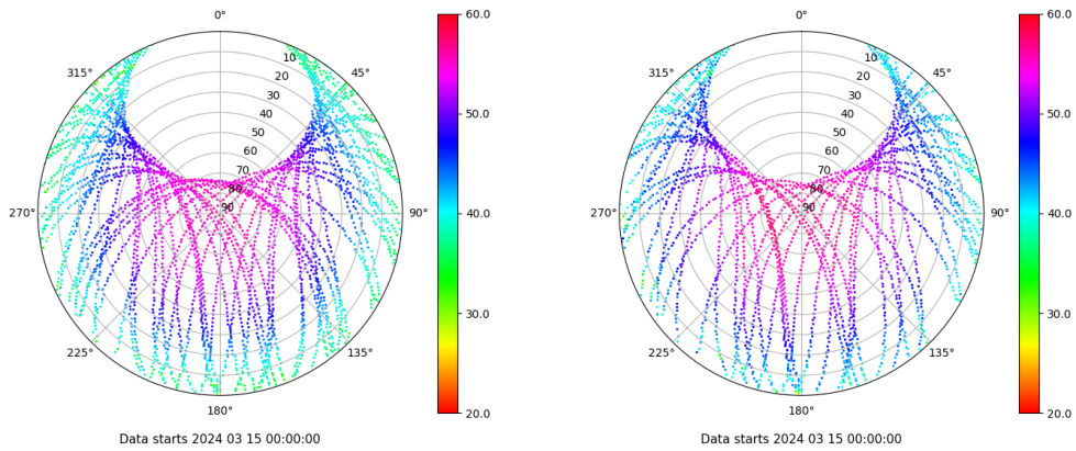
Skyplot for station XIXO. Signal to Noise S1C Data file XIXO00ESP_R_2024075.xtr Skyplot for station XIXO. Signal to Noise S2S Data file XIXO00ESP_R_2024075.xtr
