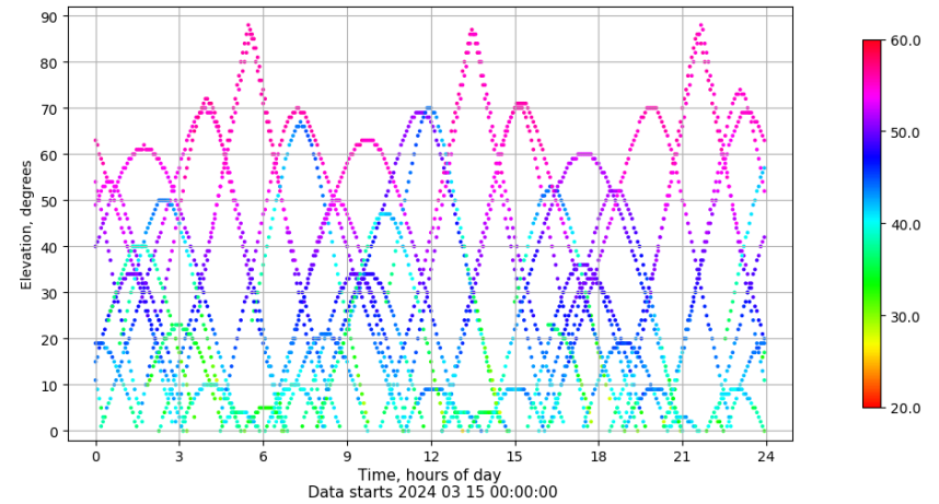
Time-elevation plot for station XIXO. Signal to Noise S1C Data file XIXO00ESP_R_2024075.xtr
