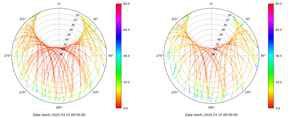
Skyplot for station XIXO. Parameter M1C Data file XIXO00ESP_R_2024075.xtr Skyplot for station XIXO. Parameter M2S Data file XIXO00ESP_R_2024075.xtr
