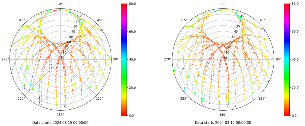
Skyplot for station XIXO. Parameter M1C Data file XIXO00ESP_R_2024075.xtr Skyplot for station XIXO. Parameter M2C Data file XIXO00ESP_R_2024075.xtr
