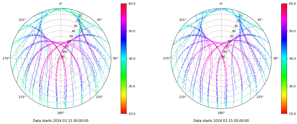
Skyplot for station XIXO. Signal to Noise S1C Data file XIXO00ESP_R_2024075.xtr Skyplot for station XIXO. Signal to Noise S2C Data file XIXO00ESP_R_2024075.xtr
