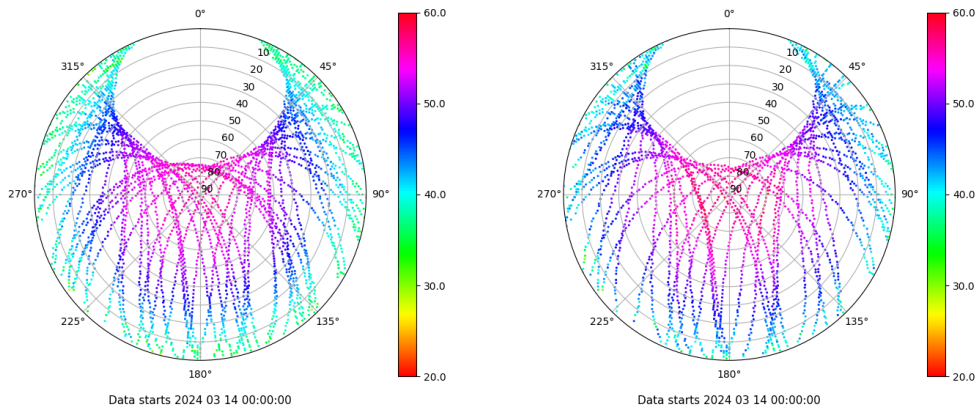
Skyplot for station XIXO. Signal to Noise S1C Data file XIXO00ESP_R_2024074.xtr Skyplot for station XIXO. Signal to Noise S2S Data file XIXO00ESP_R_2024074.xtr
