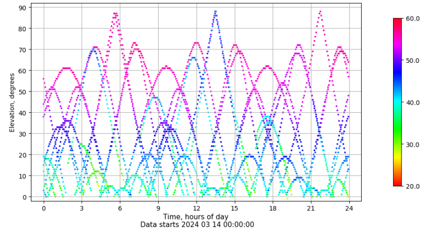
Time-elevation plot for station XIXO. Signal to Noise S1C Data file XIXO00ESP_R_2024074.xtr
