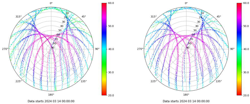
Skyplot for station XIXO. Signal to Noise S1C Data file XIXO00ESP_R_2024074.xtr Skyplot for station XIXO. Signal to Noise S2C Data file XIXO00ESP_R_2024074.xtr
