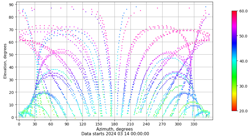
Azimuth-elevation plot for station XIXO. Signal to Noise S1C Data file XIXO00ESP_R_2024074.xtr
