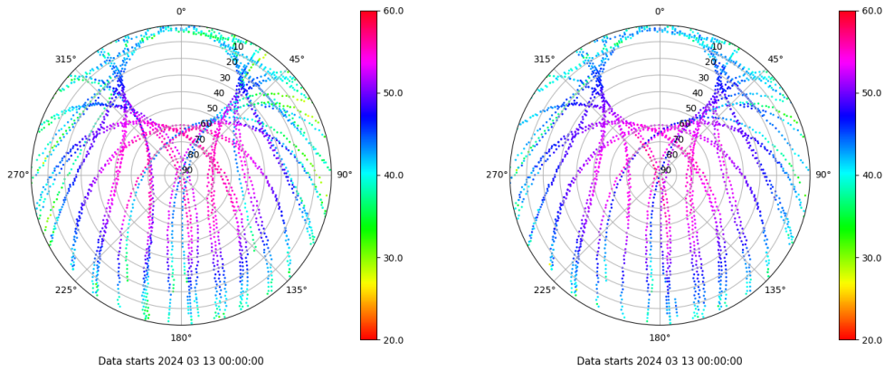
Skyplot for station XIXO. Signal to Noise S1C Data file XIXO00ESP_R_2024073.xtr Skyplot for station XIXO. Signal to Noise S2C Data file XIXO00ESP_R_2024073.xtr
