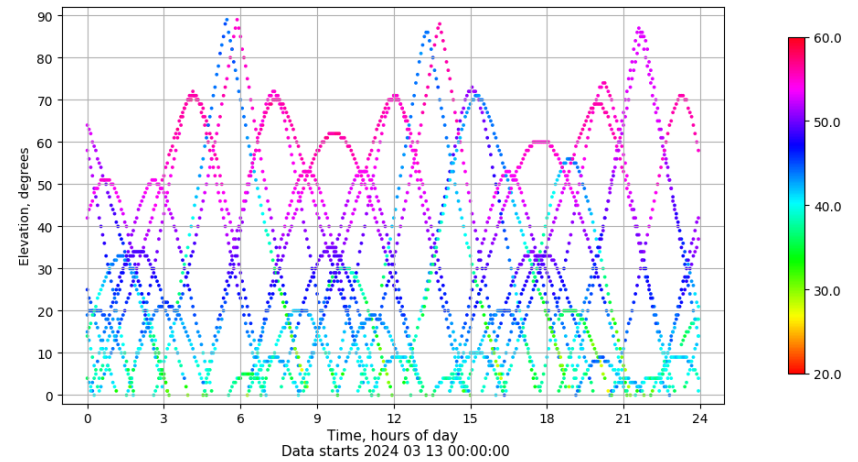
Time-elevation plot for station XIXO. Signal to Noise S1C Data file XIXO00ESP_R_2024073.xtr
