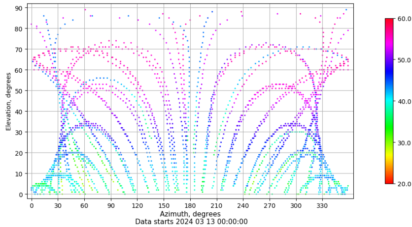
Azimuth-elevation plot for station XIXO. Signal to Noise S1C Data file XIXO00ESP_R_2024073.xtr
