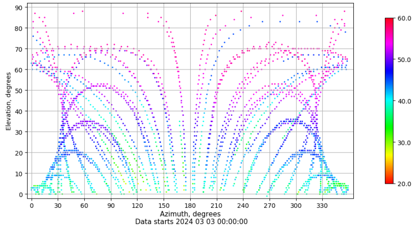
Azimuth-elevation plot for station XIXO. Signal to Noise S1C Data file XIXO00ESP_R_2024063.xtr
