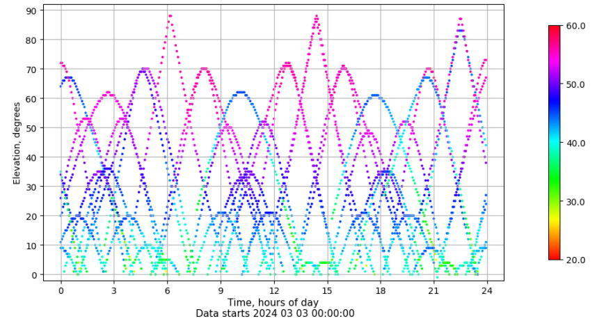
Time-elevation plot for station XIXO. Signal to Noise S1C Data file XIXO00ESP_R_2024063.xtr
