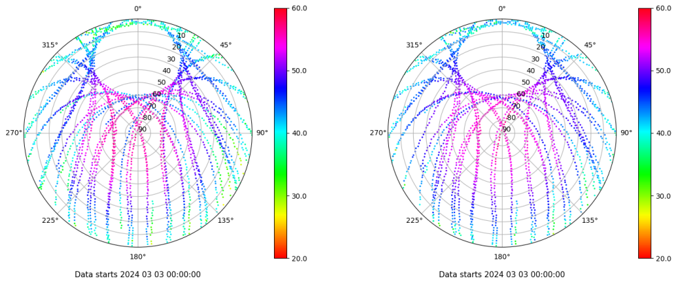
Skyplot for station XIXO. Signal to Noise S1C Data file XIXO00ESP_R_2024063.xtr Skyplot for station XIXO. Signal to Noise S2C Data file XIXO00ESP_R_2024063.xtr
