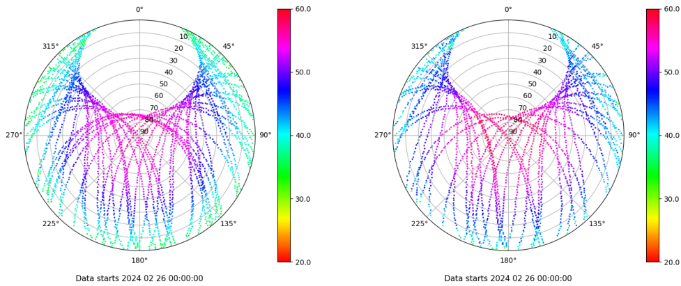
Skyplot for station XIXO. Signal to Noise S1C Data file XIXO00ESP_R_2024057.xtr Skyplot for station XIXO. Signal to Noise S2S Data file XIXO00ESP_R_2024057.xtr
