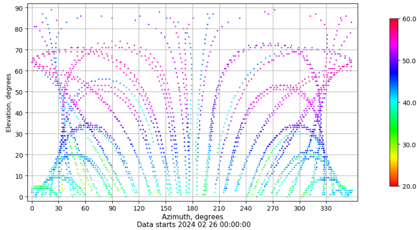
Azimuth-elevation plot for station XIXO. Signal to Noise S1C Data file XIXO00ESP_R_2024057.xtr
