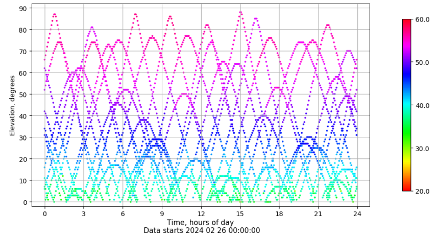
Time-elevation plot for station XIXO. Signal to Noise S1C Data file XIXO00ESP_R_2024057.xtr
