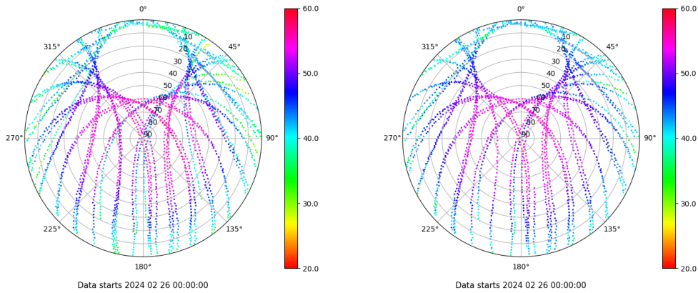
Skyplot for station XIXO. Signal to Noise S1C Data file XIXO00ESP_R_2024057.xtr Skyplot for station XIXO. Signal to Noise S2C Data file XIXO00ESP_R_2024057.xtr
