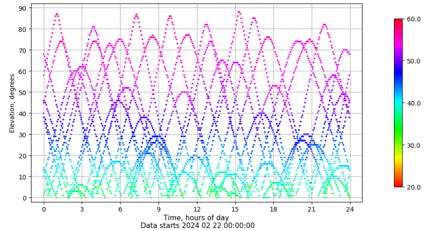
Time-elevation plot for station XIXO. Signal to Noise S1C Data file XIXO00ESP_R_2024053.xtr
