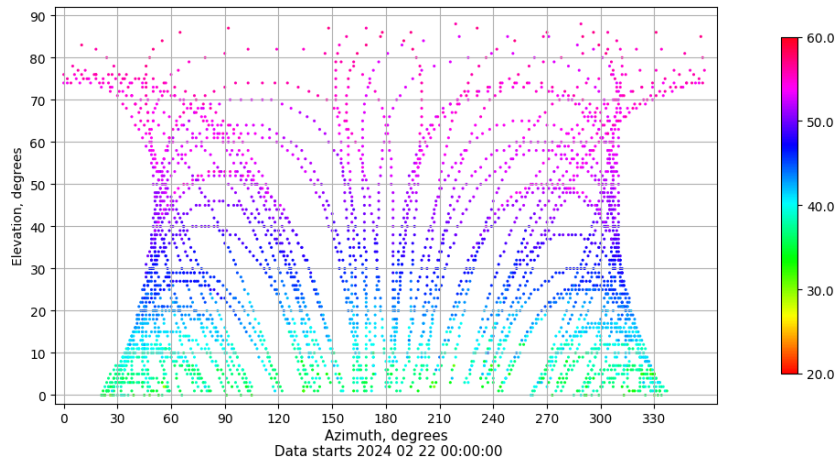
Azimuth-elevation plot for station XIXO. Signal to Noise S1C Data file XIXO00ESP_R_2024053.xtr
