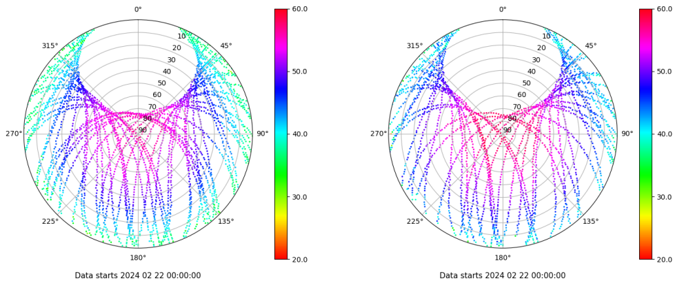
Skyplot for station XIXO. Signal to Noise S1C Data file XIXO00ESP_R_2024053.xtr Skyplot for station XIXO. Signal to Noise S2S Data file XIXO00ESP_R_2024053.xtr
