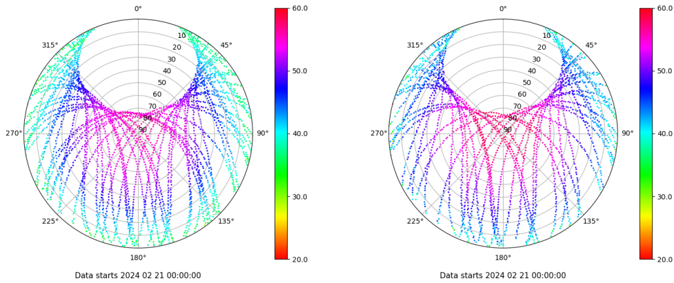
Skyplot for station XIXO. Signal to Noise S1C Data file XIXO00ESP_R_2024052.xtr Skyplot for station XIXO. Signal to Noise S2S Data file XIXO00ESP_R_2024052.xtr
