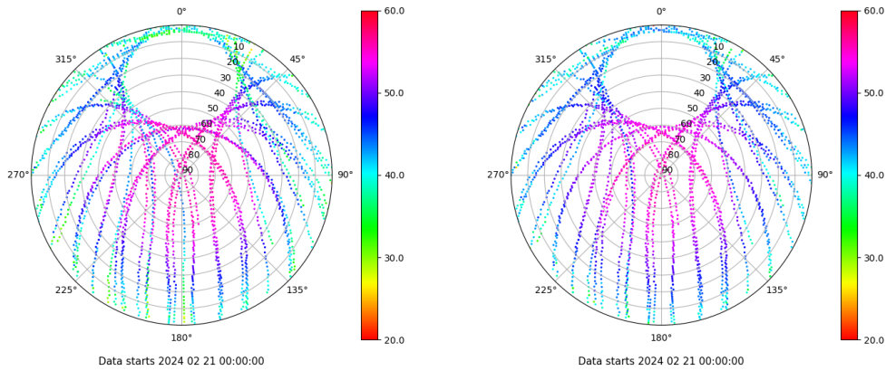
Skyplot for station XIXO. Signal to Noise S1C Data file XIXO00ESP_R_2024052.xtr Skyplot for station XIXO. Signal to Noise S2C Data file XIXO00ESP_R_2024052.xtr
