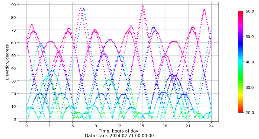
Time-elevation plot for station XIXO. Signal to Noise S1C Data file XIXO00ESP_R_2024052.xtr
