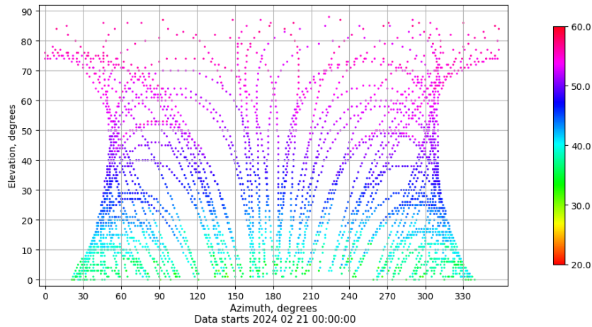
Azimuth-elevation plot for station XIXO. Signal to Noise S1C Data file XIXO00ESP_R_2024052.xtr
