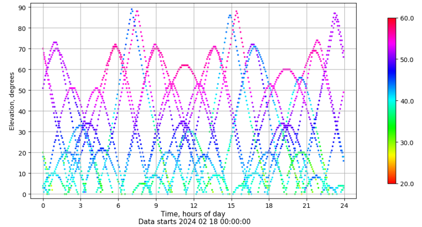
Time-elevation plot for station XIXO. Signal to Noise S1C Data file XIXO00ESP_R_2024049.xtr
