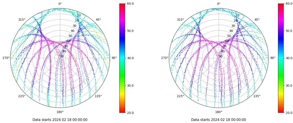
Skyplot for station XIXO. Signal to Noise S1C Data file XIXO00ESP_R_2024049.xtr Skyplot for station XIXO. Signal to Noise S2C Data file XIXO00ESP_R_2024049.xtr
