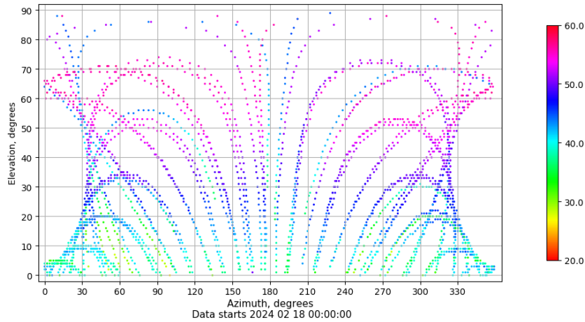
Azimuth-elevation plot for station XIXO. Signal to Noise S1C Data file XIXO00ESP_R_2024049.xtr
