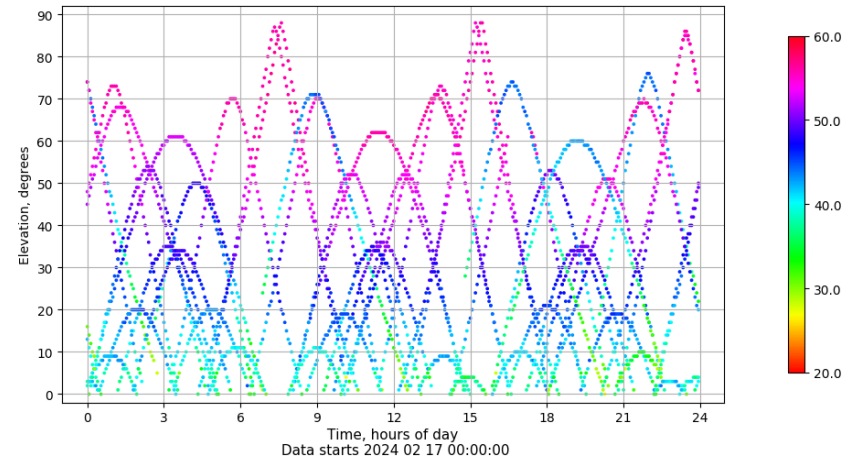
Time-elevation plot for station XIXO. Signal to Noise S1C Data file XIXO00ESP_R_2024048.xtr
