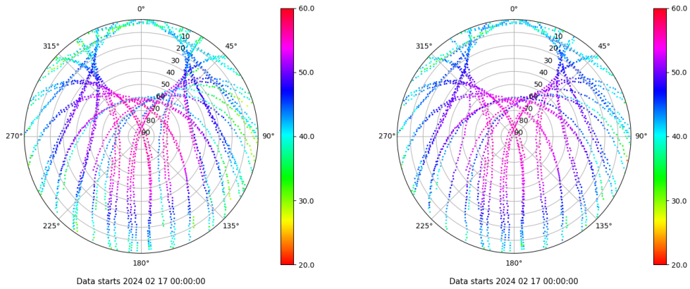
Skyplot for station XIXO. Signal to Noise S1C Data file XIXO00ESP_R_2024048.xtr Skyplot for station XIXO. Signal to Noise S2C Data file XIXO00ESP_R_2024048.xtr
