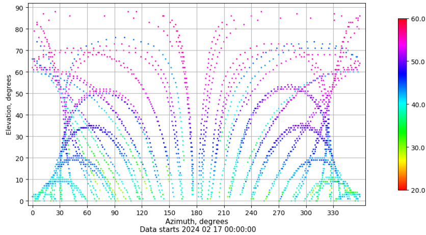
Azimuth-elevation plot for station XIXO. Signal to Noise S1C Data file XIXO00ESP_R_2024048.xtr
