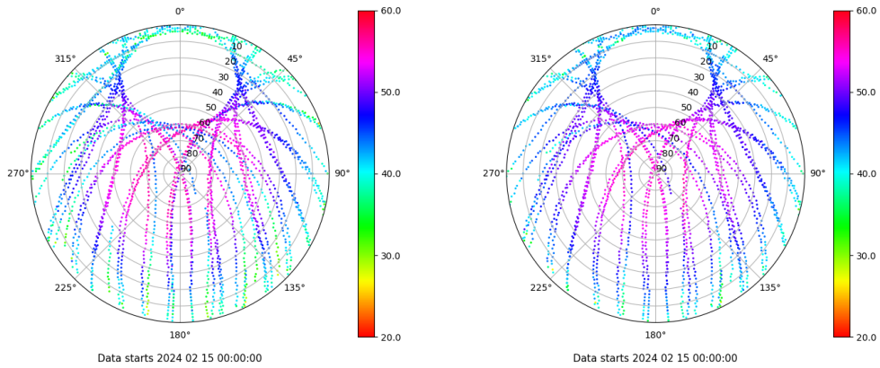
Skyplot for station XIXO. Signal to Noise S1C Data file XIXO00ESP_R_2024046.xtr Skyplot for station XIXO. Signal to Noise S2C Data file XIXO00ESP_R_2024046.xtr
