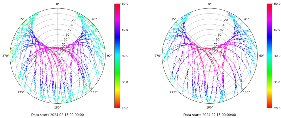
Skyplot for station XIXO. Signal to Noise S1C Data file XIXO00ESP_R_2024046.xtr Skyplot for station XIXO. Signal to Noise S2S Data file XIXO00ESP_R_2024046.xtr
