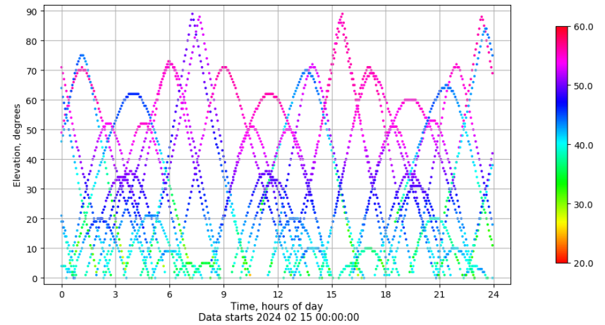
Time-elevation plot for station XIXO. Signal to Noise S1C Data file XIXO00ESP_R_2024046.xtr
