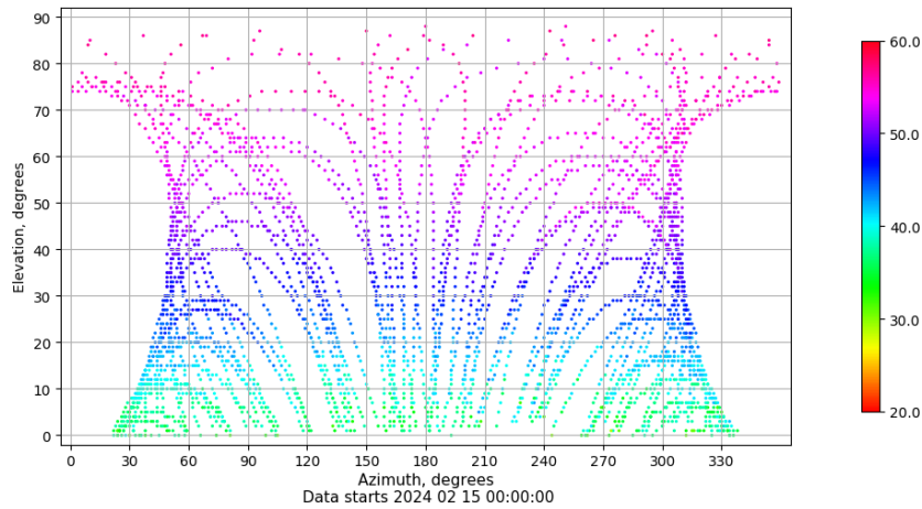
Azimuth-elevation plot for station XIXO. Signal to Noise S1C Data file XIXO00ESP_R_2024046.xtr
