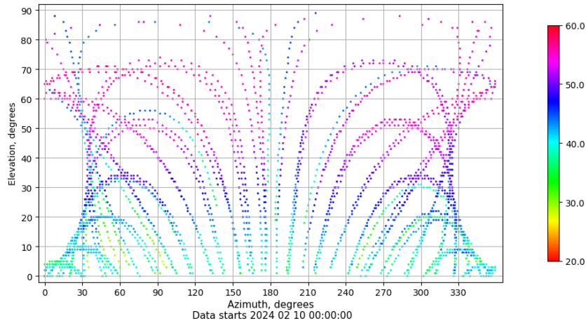
Azimuth-elevation plot for station XIXO. Signal to Noise S1C Data file XIXO00ESP_R_2024041.xtr
