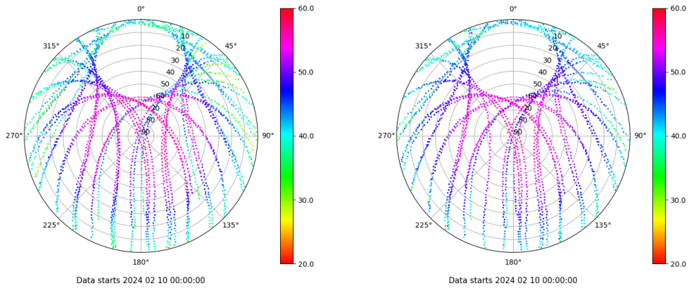
Skyplot for station XIXO. Signal to Noise S1C Data file XIXO00ESP_R_2024041.xtr Skyplot for station XIXO. Signal to Noise S2C Data file XIXO00ESP_R_2024041.xtr
