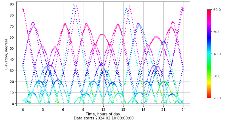
Time-elevation plot for station XIXO. Signal to Noise S1C Data file XIXO00ESP_R_2024041.xtr
