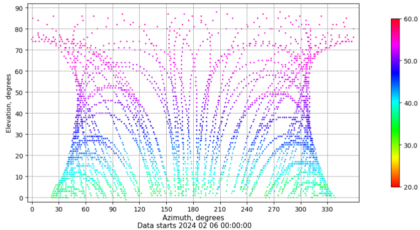
Azimuth-elevation plot for station XIXO. Signal to Noise S1C Data file XIXO00ESP_R_2024037.xtr
