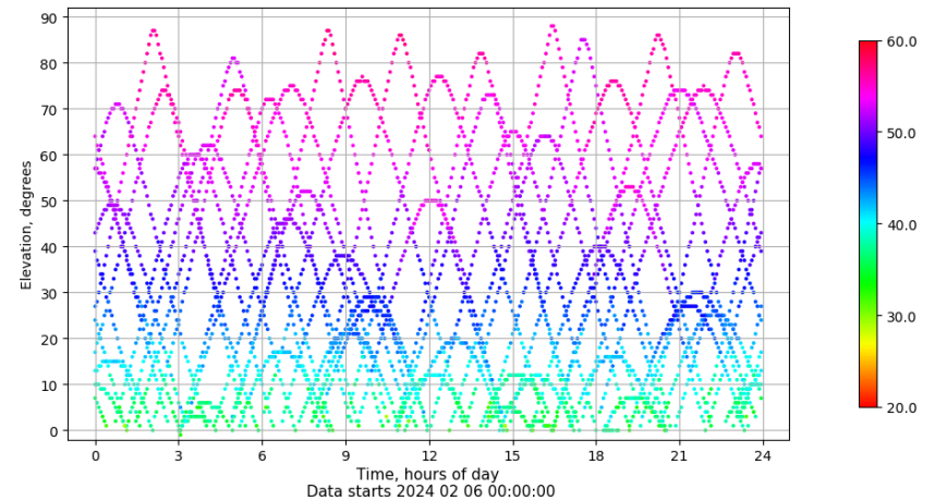
Time-elevation plot for station XIXO. Signal to Noise S1C Data file XIXO00ESP_R_2024037.xtr
