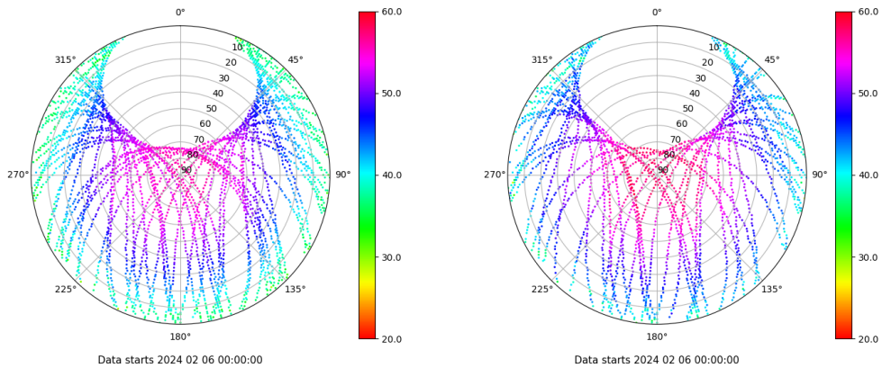
Skyplot for station XIXO. Signal to Noise S1C Data file XIXO00ESP_R_2024037.xtr Skyplot for station XIXO. Signal to Noise S2S Data file XIXO00ESP_R_2024037.xtr
