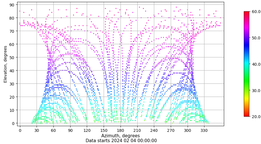
Azimuth-elevation plot for station XIXO. Signal to Noise S1C Data file XIXO00ESP_R_2024035.xtr
