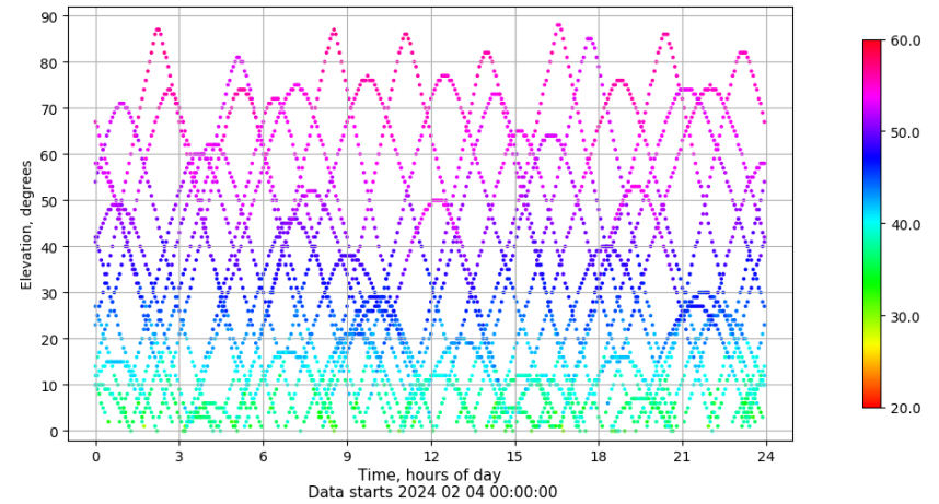
Time-elevation plot for station XIXO. Signal to Noise S1C Data file XIXO00ESP_R_2024035.xtr
