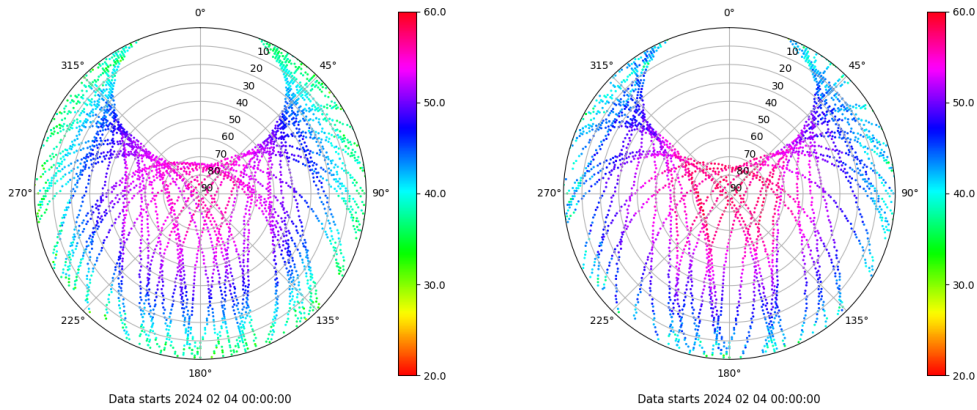
Skyplot for station XIXO. Signal to Noise S1C Data file XIXO00ESP_R_2024035.xtr Skyplot for station XIXO. Signal to Noise S2S Data file XIXO00ESP_R_2024035.xtr
