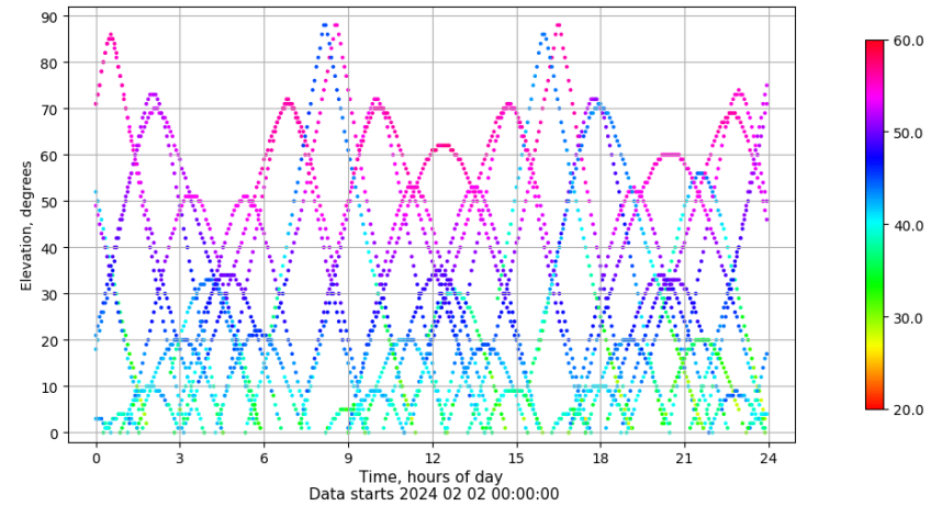
Time-elevation plot for station XIXO. Signal to Noise S1C Data file XIXO00ESP_R_2024033.xtr
