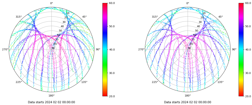
Skyplot for station XIXO. Signal to Noise S1C Data file XIXO00ESP_R_2024033.xtr Skyplot for station XIXO. Signal to Noise S2C Data file XIXO00ESP_R_2024033.xtr
