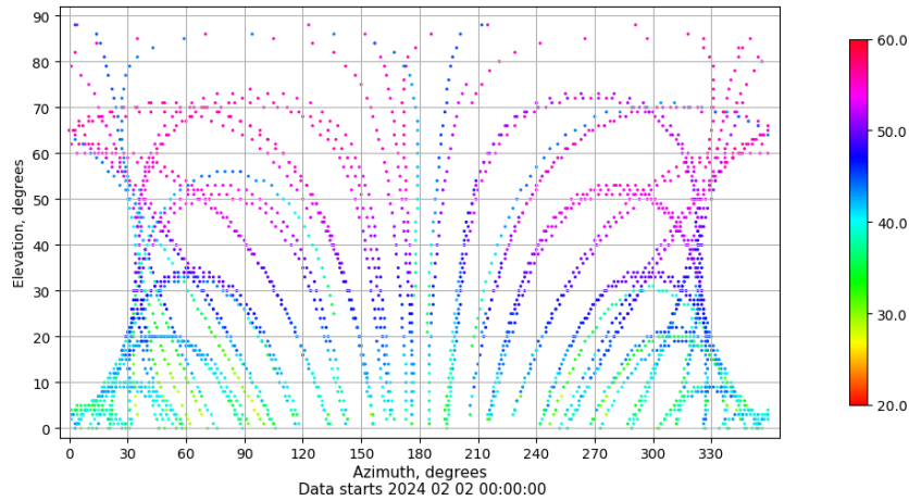
Azimuth-elevation plot for station XIXO. Signal to Noise S1C Data file XIXO00ESP_R_2024033.xtr
