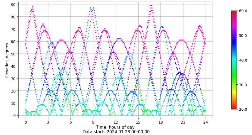
Time-elevation plot for station XIXO. Signal to Noise S1C Data file XIXO00ESP_R_2024028.xtr
