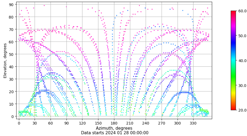
Azimuth-elevation plot for station XIXO. Signal to Noise S1C Data file XIXO00ESP_R_2024028.xtr
