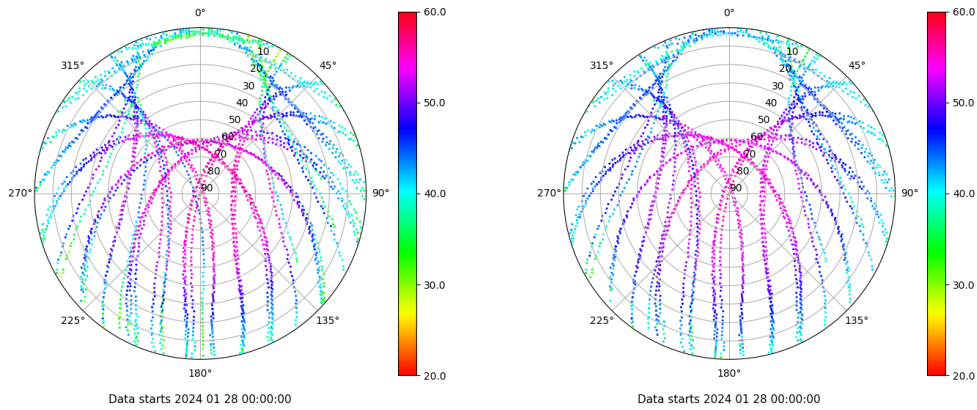
Skyplot for station XIXO. Signal to Noise S1C Data file XIXO00ESP_R_2024028.xtr Skyplot for station XIXO. Signal to Noise S2C Data file XIXO00ESP_R_2024028.xtr
