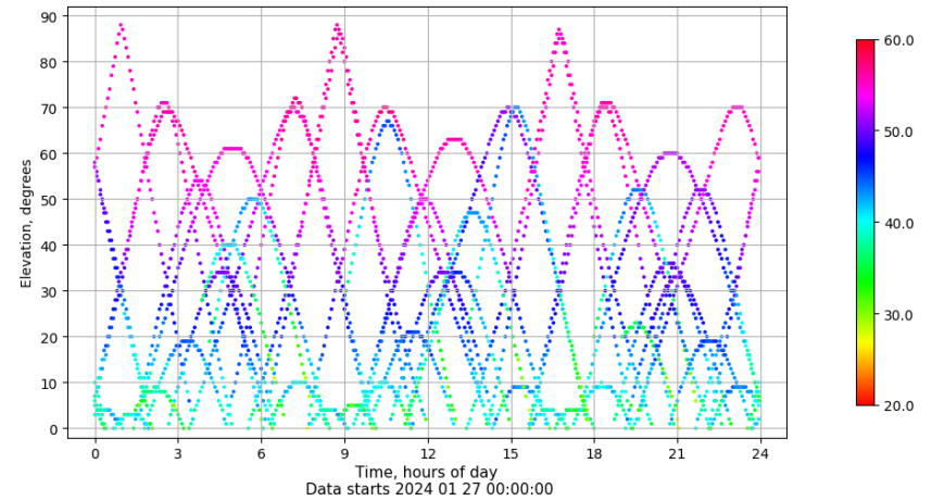
Time-elevation plot for station XIXO. Signal to Noise S1C Data file XIXO00ESP_R_2024027.xtr
