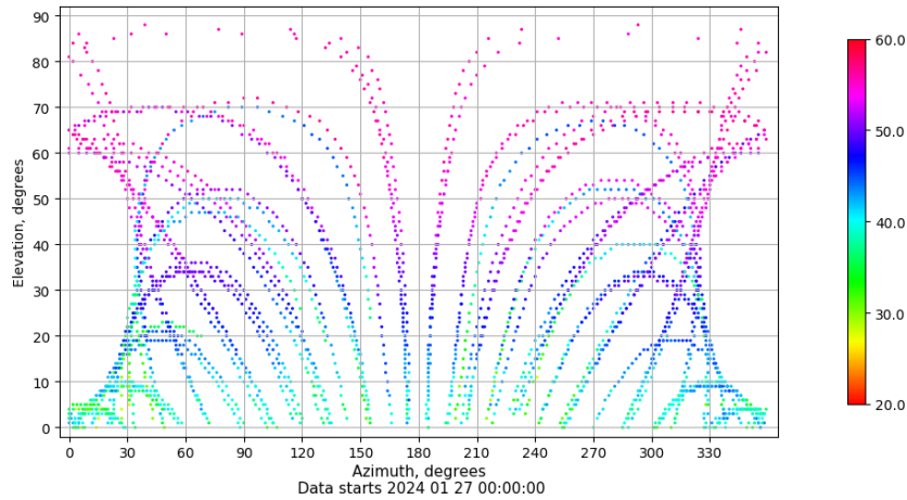
Azimuth-elevation plot for station XIXO. Signal to Noise S1C Data file XIXO00ESP_R_2024027.xtr
