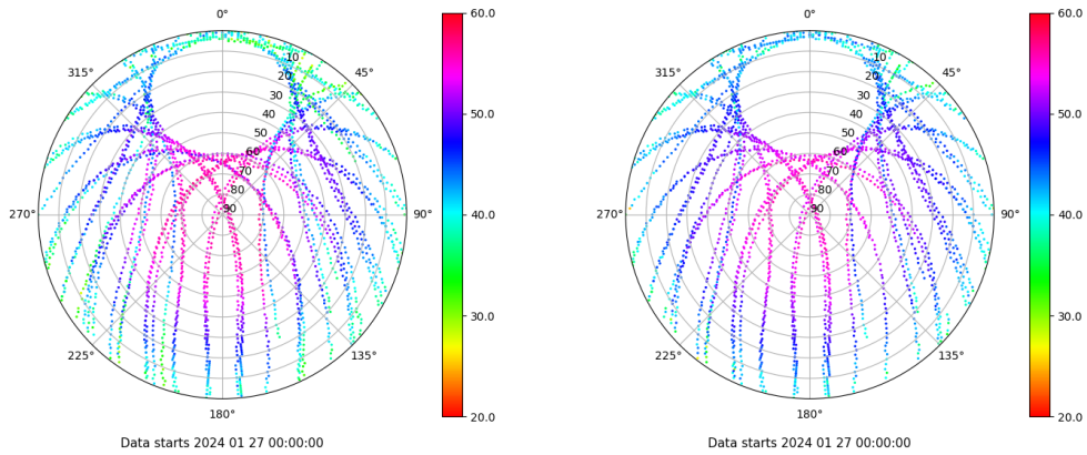
Skyplot for station XIXO. Signal to Noise S1C Data file XIXO00ESP_R_2024027.xtr Skyplot for station XIXO. Signal to Noise S2C Data file XIXO00ESP_R_2024027.xtr
