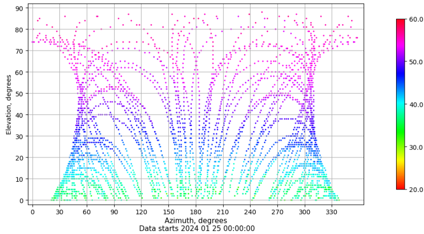
Azimuth-elevation plot for station XIXO. Signal to Noise S1C Data file XIXO00ESP_R_2024025.xtr
