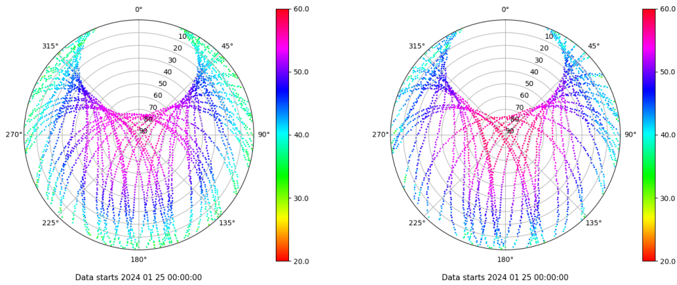
Skyplot for station XIXO. Signal to Noise S1C Data file XIXO00ESP_R_2024025.xtr Skyplot for station XIXO. Signal to Noise S2S Data file XIXO00ESP_R_2024025.xtr
