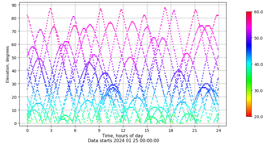
Time-elevation plot for station XIXO. Signal to Noise S1C Data file XIXO00ESP_R_2024025.xtr
