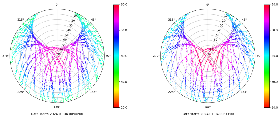
Skyplot for station XIXO. Signal to Noise S1C Data file XIXO00ESP_R_2024004.xtr Skyplot for station XIXO. Signal to Noise S2S Data file XIXO00ESP_R_2024004.xtr
