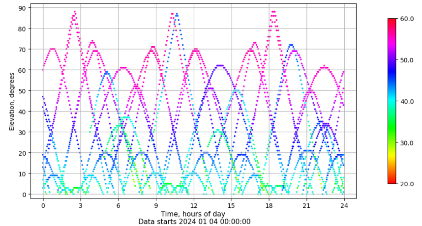
Time-elevation plot for station XIXO. Signal to Noise S1C Data file XIXO00ESP_R_2024004.xtr
