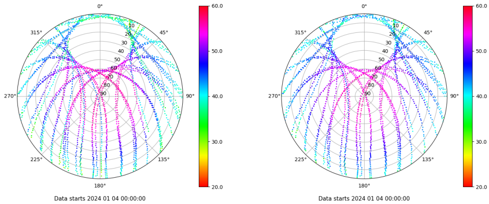
Skyplot for station XIXO. Signal to Noise S1C Data file XIXO00ESP_R_2024004.xtr Skyplot for station XIXO. Signal to Noise S2C Data file XIXO00ESP_R_2024004.xtr
