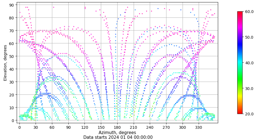
Azimuth-elevation plot for station XIXO. Signal to Noise S1C Data file XIXO00ESP_R_2024004.xtr
