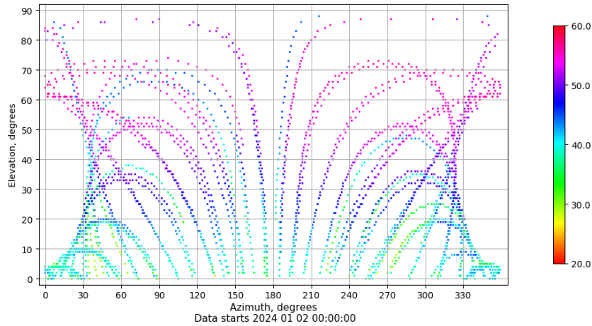
Azimuth-elevation plot for station XIXO. Signal to Noise S1C Data file XIXO00ESP_R_2024002.xtr
