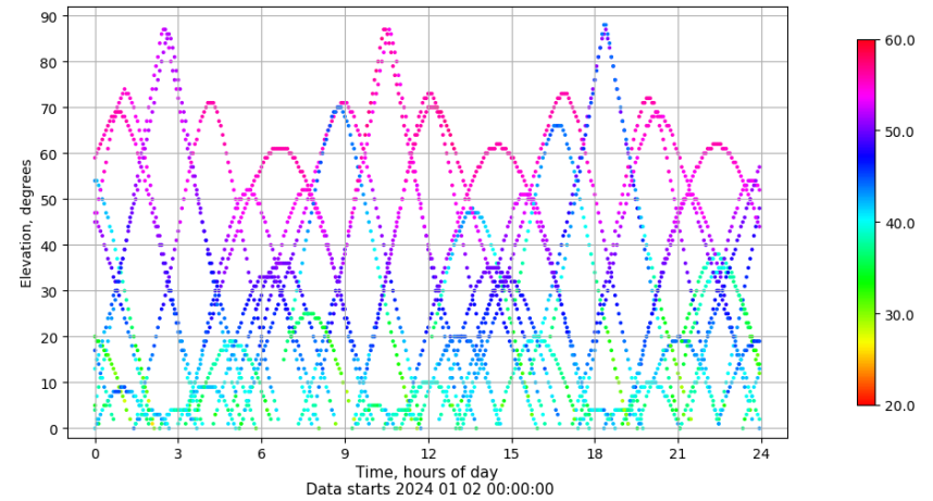
Time-elevation plot for station XIXO. Signal to Noise S1C Data file XIXO00ESP_R_2024002.xtr
