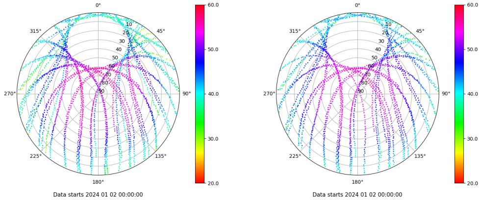
Skyplot for station XIXO. Signal to Noise S1C Data file XIXO00ESP_R_2024002.xtr Skyplot for station XIXO. Signal to Noise S2C Data file XIXO00ESP_R_2024002.xtr
