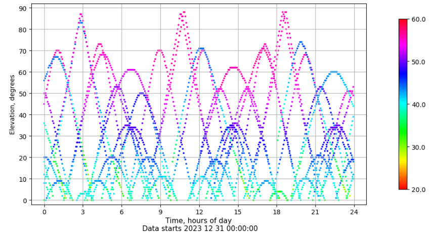
Time-elevation plot for station XIXO. Signal to Noise S1C Data file XIXO00ESP_R_2023365.xtr
