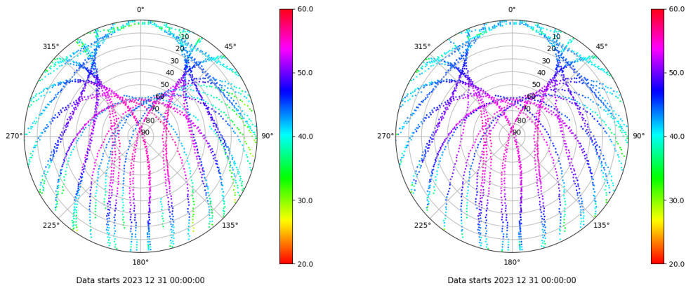
Skyplot for station XIXO. Signal to Noise S1C Data file XIXO00ESP_R_2023365.xtr Skyplot for station XIXO. Signal to Noise S2C Data file XIXO00ESP_R_2023365.xtr
