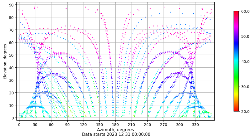
Azimuth-elevation plot for station XIXO. Signal to Noise S1C Data file XIXO00ESP_R_2023365.xtr
