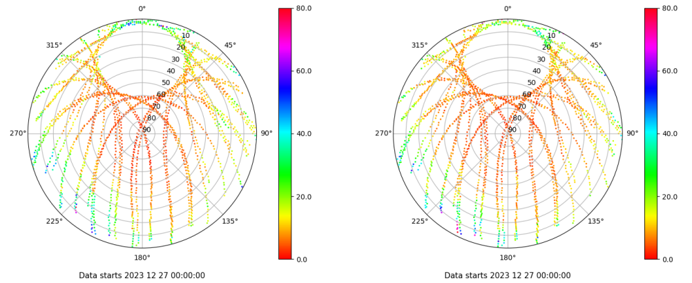
Skyplot for station XIXO. Parameter M1C Data file XIXO00ESP_R_2023361.xtr Skyplot for station XIXO. Parameter M2C Data file XIXO00ESP_R_2023361.xtr
