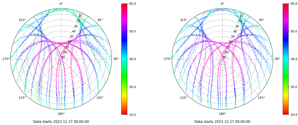
Skyplot for station XIXO. Signal to Noise S1C Data file XIXO00ESP_R_2023361.xtr Skyplot for station XIXO. Signal to Noise S2C Data file XIXO00ESP_R_2023361.xtr
