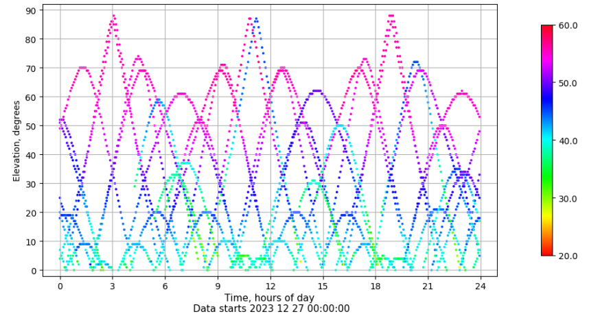
Time-elevation plot for station XIXO. Signal to Noise S1C Data file XIXO00ESP_R_2023361.xtr
