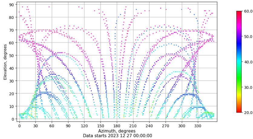
Azimuth-elevation plot for station XIXO. Signal to Noise S1C Data file XIXO00ESP_R_2023361.xtr
