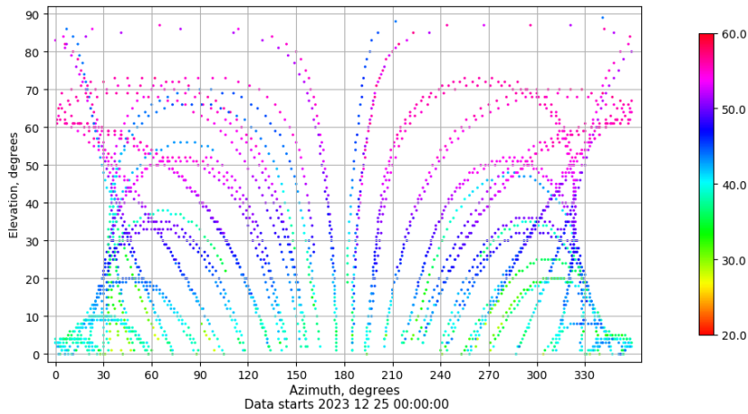
Azimuth-elevation plot for station XIXO. Signal to Noise S1C Data file XIXO00ESP_R_2023359.xtr
