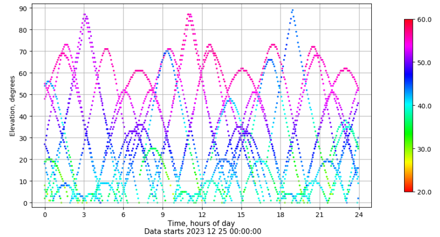
Time-elevation plot for station XIXO. Signal to Noise S1C Data file XIXO00ESP_R_2023359.xtr
