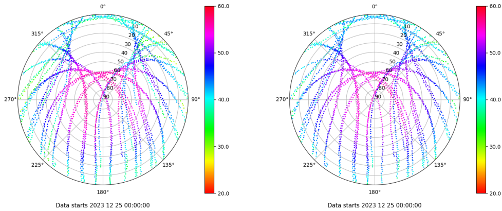
Skyplot for station XIXO. Signal to Noise S1C Data file XIXO00ESP_R_2023359.xtr Skyplot for station XIXO. Signal to Noise S2C Data file XIXO00ESP_R_2023359.xtr
