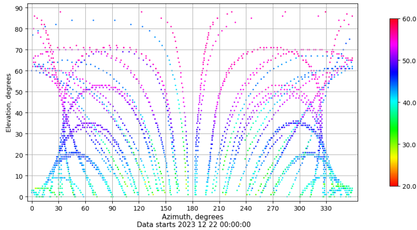
Azimuth-elevation plot for station XIXO. Signal to Noise S1C Data file XIXO00ESP_R_2023356.xtr
