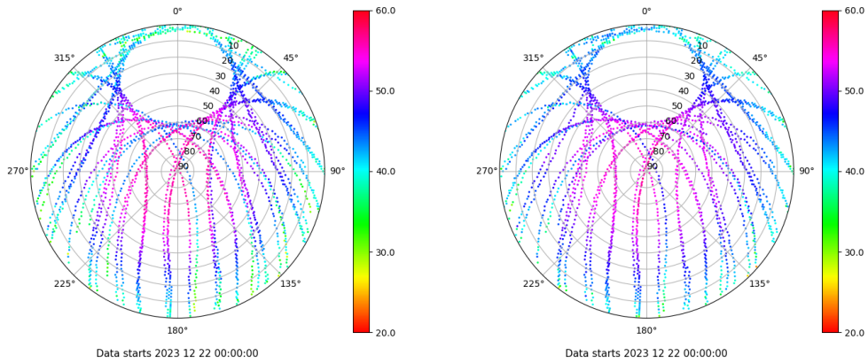
Skyplot for station XIXO. Signal to Noise S1C Data file XIXO00ESP_R_2023356.xtr Skyplot for station XIXO. Signal to Noise S2C Data file XIXO00ESP_R_2023356.xtr
