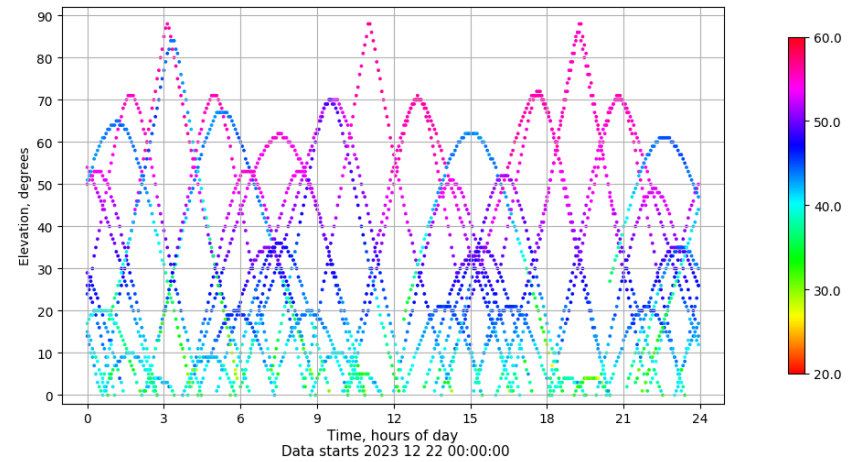
Time-elevation plot for station XIXO. Signal to Noise S1C Data file XIXO00ESP_R_2023356.xtr
