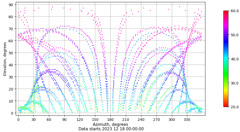
Azimuth-elevation plot for station XIXO. Signal to Noise S1C Data file XIXO00ESP_R_2023352.xtr
