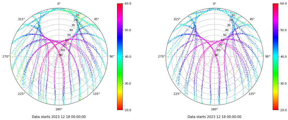
Skyplot for station XIXO. Signal to Noise S1C Data file XIXO00ESP_R_2023352.xtr Skyplot for station XIXO. Signal to Noise S2C Data file XIXO00ESP_R_2023352.xtr
