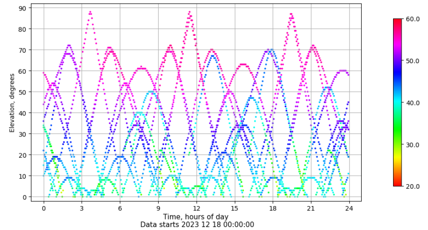
Time-elevation plot for station XIXO. Signal to Noise S1C Data file XIXO00ESP_R_2023352.xtr
