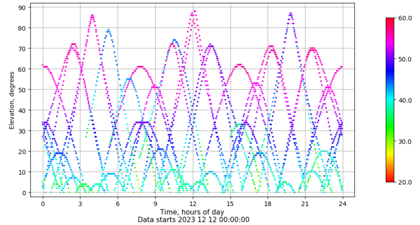
Time-elevation plot for station XIXO. Signal to Noise S1C Data file XIXO00ESP_R_2023346.xtr
