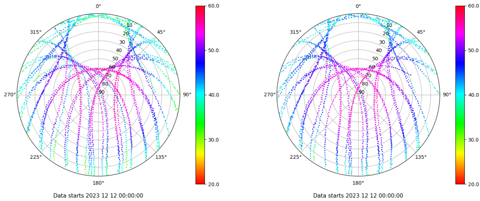
Skyplot for station XIXO. Signal to Noise S1C Data file XIXO00ESP_R_2023346.xtr Skyplot for station XIXO. Signal to Noise S2C Data file XIXO00ESP_R_2023346.xtr
