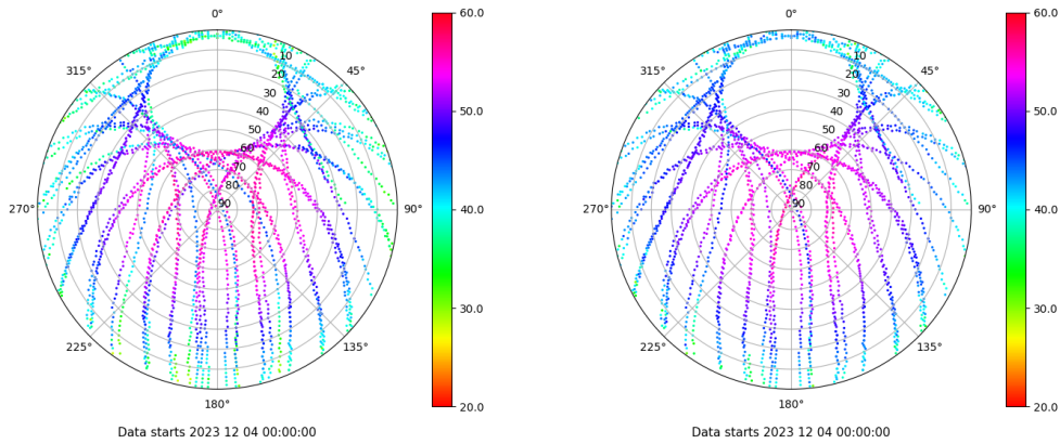
Skyplot for station XIXO. Signal to Noise S1C Data file XIXO00ESP_R_2023338.xtr Skyplot for station XIXO. Signal to Noise S2C Data file XIXO00ESP_R_2023338.xtr
