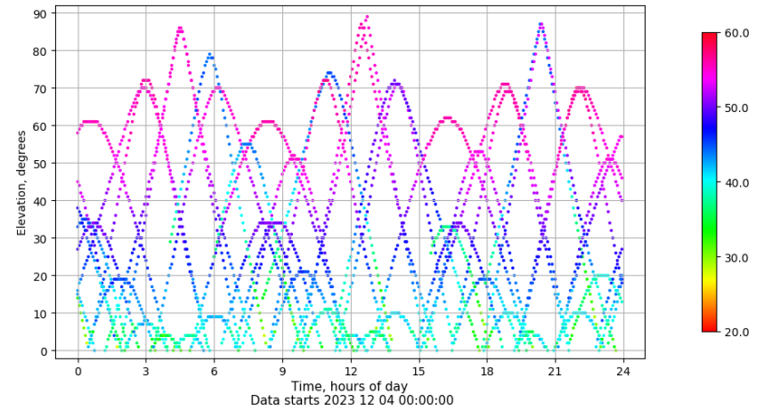
Time-elevation plot for station XIXO. Signal to Noise S1C Data file XIXO00ESP_R_2023338.xtr
