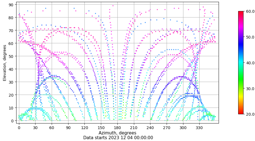
Azimuth-elevation plot for station XIXO. Signal to Noise S1C Data file XIXO00ESP_R_2023338.xtr
