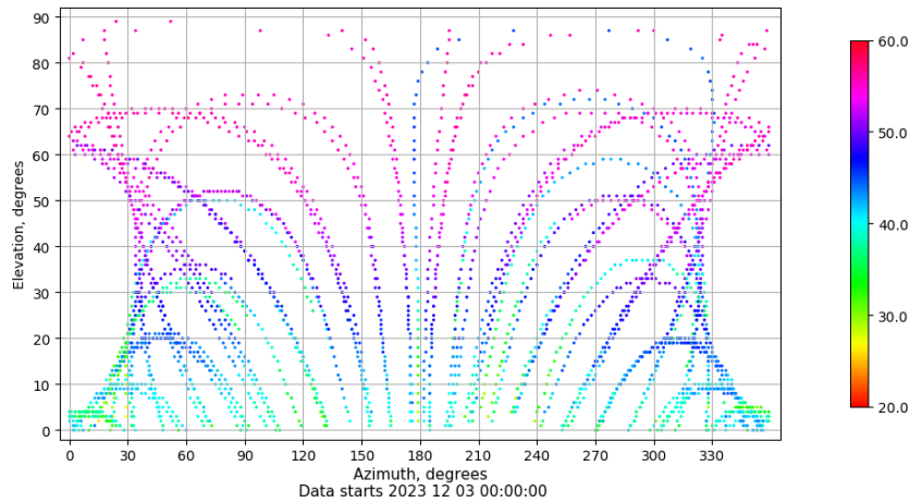
Azimuth-elevation plot for station XIXO. Signal to Noise S1C Data file XIXO00ESP_R_2023337.xtr
