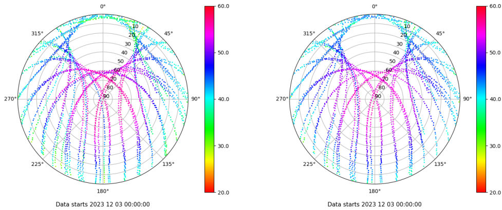
Skyplot for station XIXO. Signal to Noise S1C Data file XIXO00ESP_R_2023337.xtr Skyplot for station XIXO. Signal to Noise S2C Data file XIXO00ESP_R_2023337.xtr
