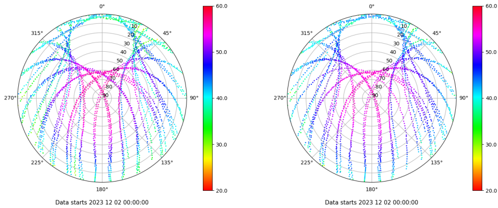
Skyplot for station XIXO. Signal to Noise S1C Data file XIXO00ESP_R_2023336.xtr Skyplot for station XIXO. Signal to Noise S2C Data file XIXO00ESP_R_2023336.xtr
