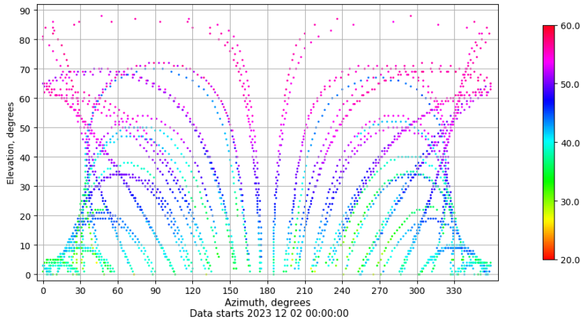
Azimuth-elevation plot for station XIXO. Signal to Noise S1C Data file XIXO00ESP_R_2023336.xtr
