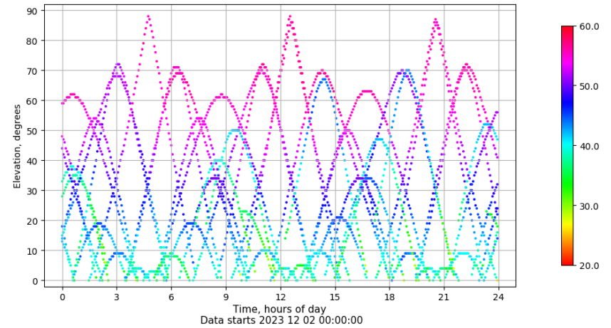
Time-elevation plot for station XIXO. Signal to Noise S1C Data file XIXO00ESP_R_2023336.xtr
