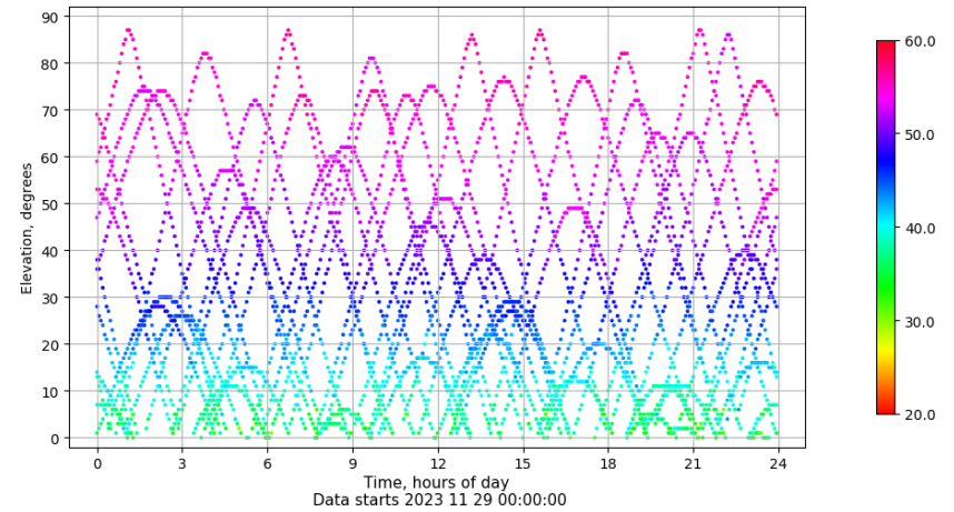
Time-elevation plot for station XIXO. Signal to Noise S1C Data file XIXO00ESP_R_2023333.xtr
