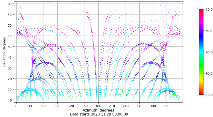
Azimuth-elevation plot for station XIXO. Signal to Noise S1C Data file XIXO00ESP_R_2023333.xtr
