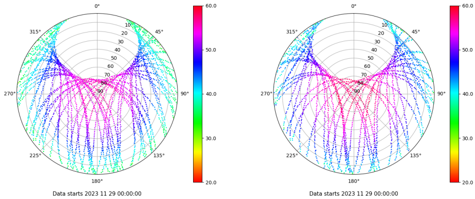
Skyplot for station XIXO. Signal to Noise S1C Data file XIXO00ESP_R_2023333.xtr Skyplot for station XIXO. Signal to Noise S2S Data file XIXO00ESP_R_2023333.xtr
