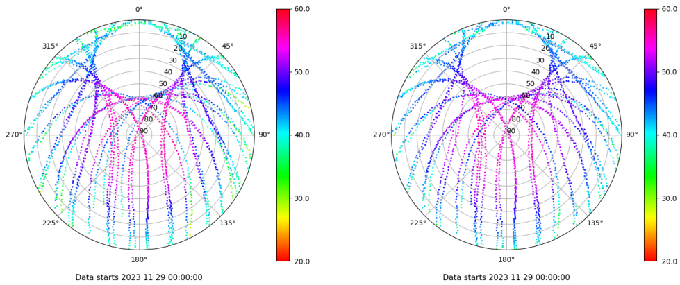
Skyplot for station XIXO. Signal to Noise S1C Data file XIXO00ESP_R_2023333.xtr Skyplot for station XIXO. Signal to Noise S2C Data file XIXO00ESP_R_2023333.xtr
