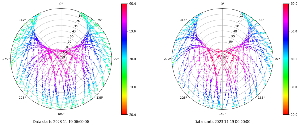
Skyplot for station XIXO. Signal to Noise S1C Data file XIXO00ESP_R_2023323.xtr Skyplot for station XIXO. Signal to Noise S2S Data file XIXO00ESP_R_2023323.xtr
