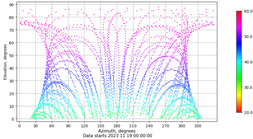
Azimuth-elevation plot for station XIXO. Signal to Noise S1C Data file XIXO00ESP_R_2023323.xtr
