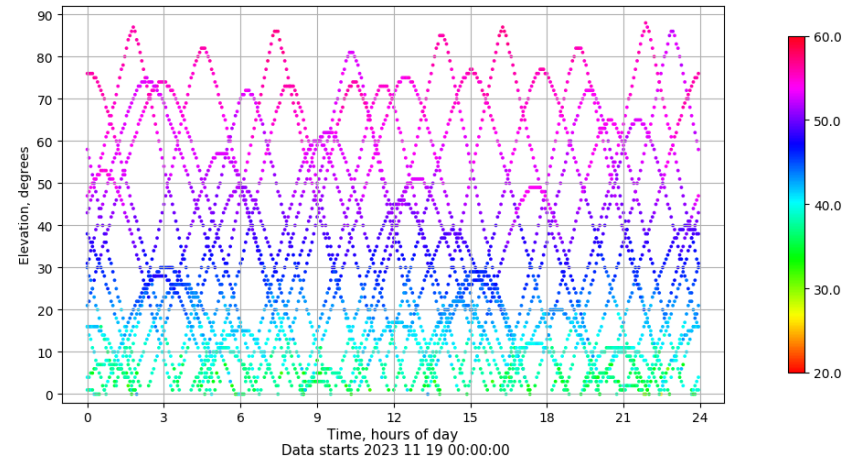
Time-elevation plot for station XIXO. Signal to Noise S1C Data file XIXO00ESP_R_2023323.xtr
