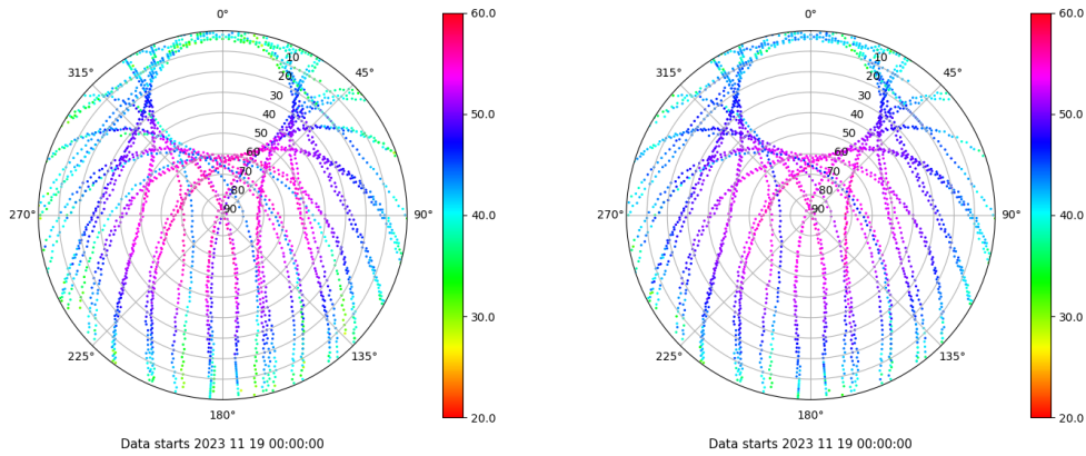
Skyplot for station XIXO. Signal to Noise S1C Data file XIXO00ESP_R_2023323.xtr Skyplot for station XIXO. Signal to Noise S2C Data file XIXO00ESP_R_2023323.xtr
