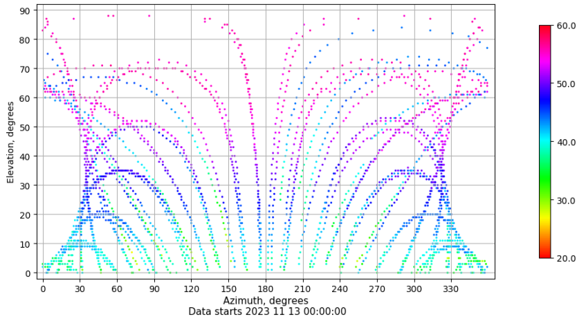
Azimuth-elevation plot for station XIXO. Signal to Noise S1C Data file XIXO00ESP_R_2023317.xtr
