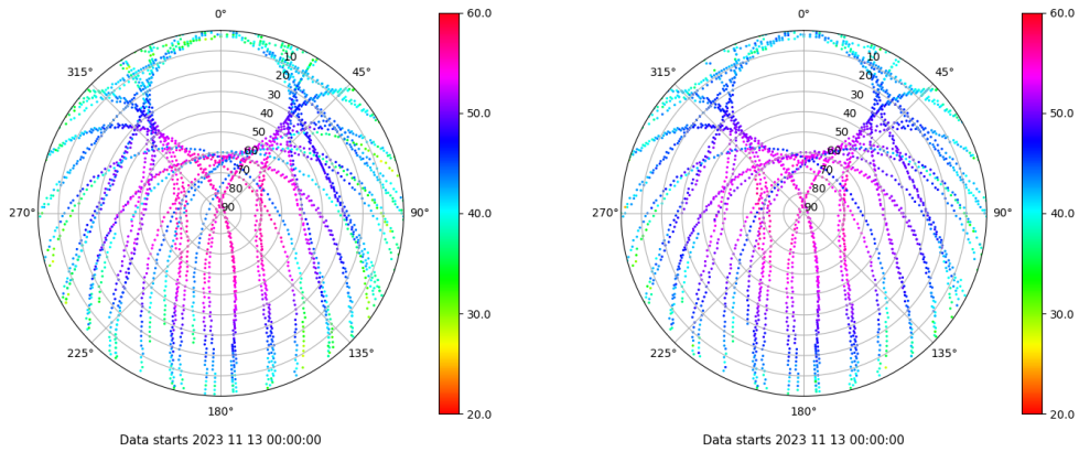
Skyplot for station XIXO. Signal to Noise S1C Data file XIXO00ESP_R_2023317.xtr Skyplot for station XIXO. Signal to Noise S2C Data file XIXO00ESP_R_2023317.xtr
