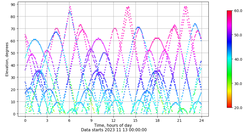
Time-elevation plot for station XIXO. Signal to Noise S1C Data file XIXO00ESP_R_2023317.xtr
