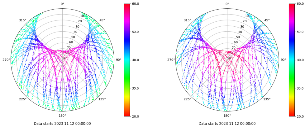
Skyplot for station XIXO. Signal to Noise S1C Data file XIXO00ESP_R_2023316.xtr Skyplot for station XIXO. Signal to Noise S2S Data file XIXO00ESP_R_2023316.xtr
