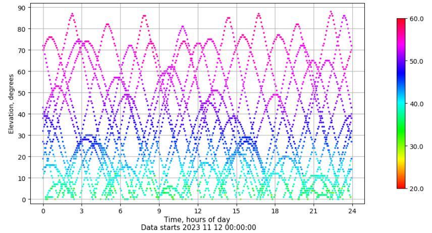
Time-elevation plot for station XIXO. Signal to Noise S1C Data file XIXO00ESP_R_2023316.xtr
