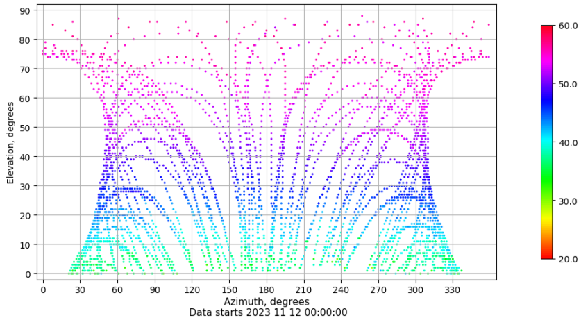
Azimuth-elevation plot for station XIXO. Signal to Noise S1C Data file XIXO00ESP_R_2023316.xtr
